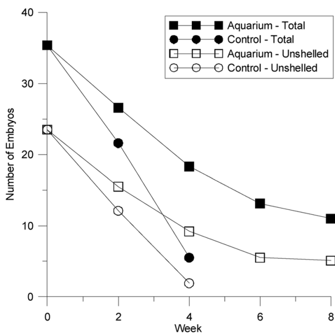
Figure 3. Embryo numbers in the control and in an aquarium declined substantially over the duration of the experiment. The decline in the aquarium was slower and not as pronounced, and leveled off at 8 weeks.
