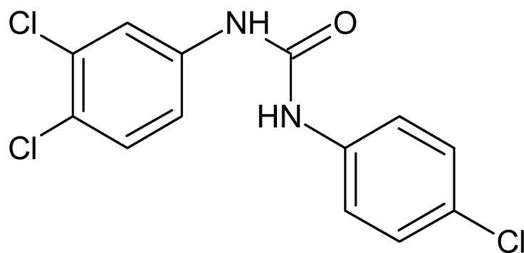
Figure 1. Chemical structure of triclocarban (TCC) .
