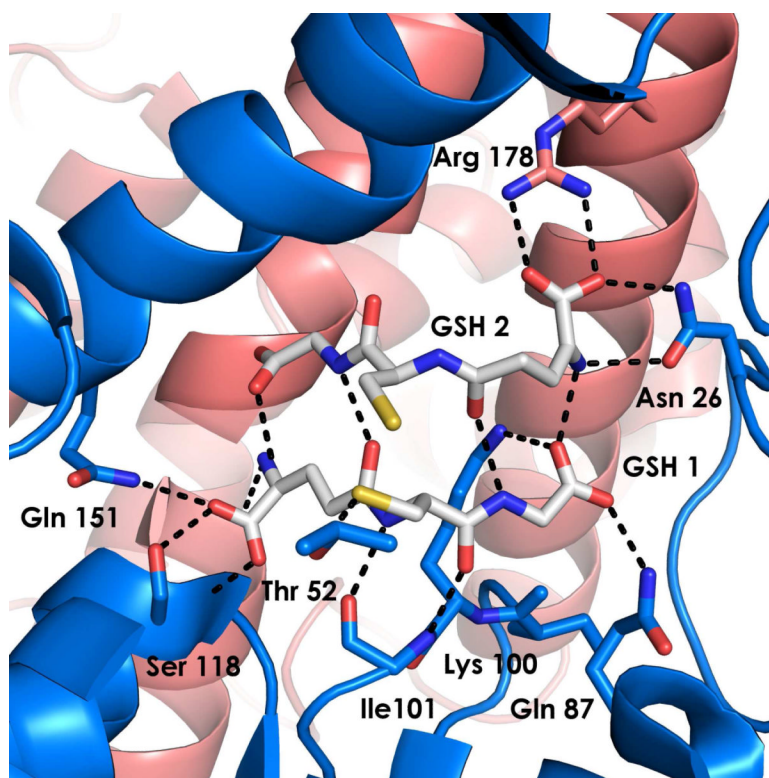
Figure 4. Details of the potential hydrogen-bonding interactions of the two GSH molecules in the active site of YghU. The primary subunit is shown in blue and the opposing subunit is shown in red. The two GSH molecules are shown in stick representation. The sulfur atoms are shown in yellow
