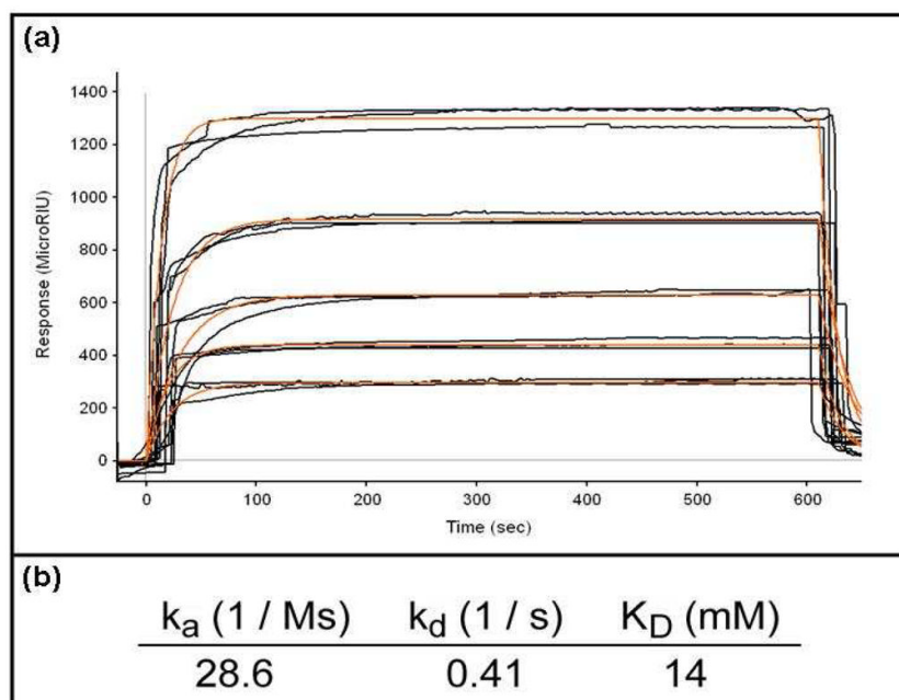
Figure 4. Affinity of dextran for CTB
