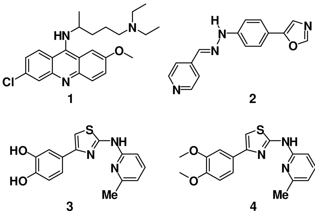
Figure 1. Structures of small molecules with antiprion properties.
