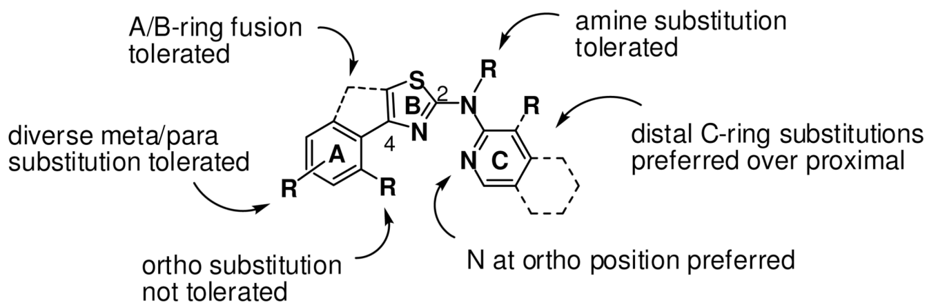
Figure 2. Summary of structure-antiprion activity relationships for 2-aminothiazole analogs. The three rings are arbitrarily denoted A, B, and C for convenience.
