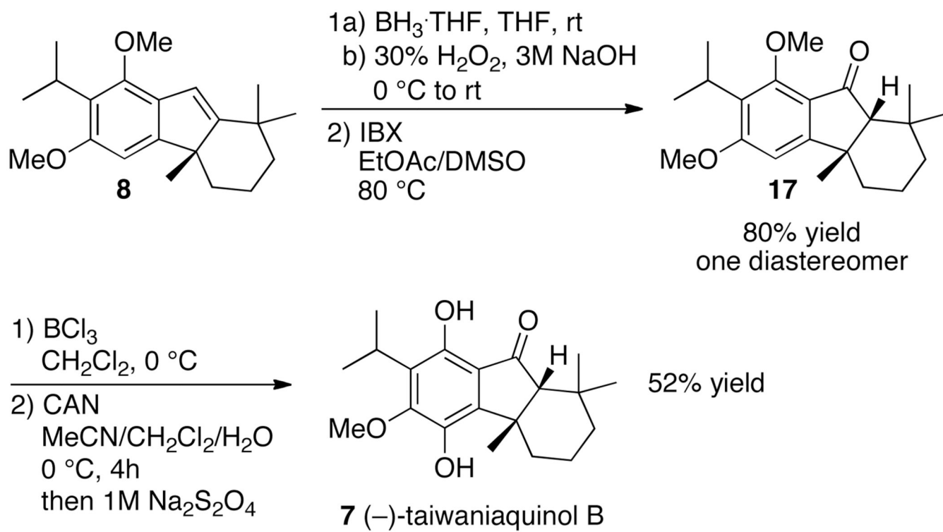
Scheme 5. Synthesis of (-)-Taiwaniaquinol B (7)
