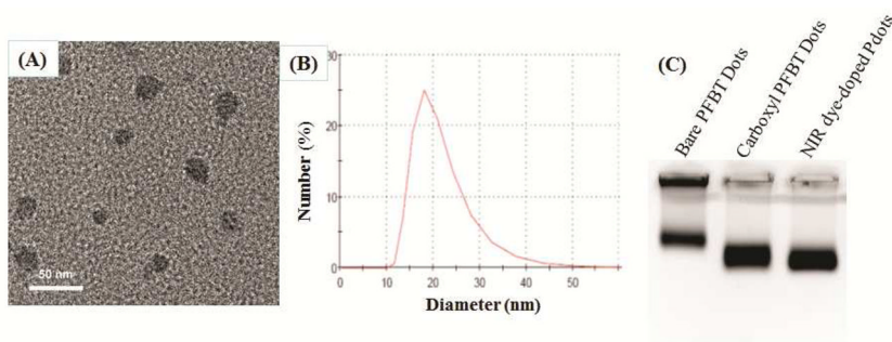
Figure 1. Characterization of NIR775 dye-doped PFBT Pdts. (A) TEM image of NIR775 dye-doped Pdts; the average diameter of the Pdts was 18 nm. (B) Average diameter of NIR775 dye-doped Pdts measured by dynamic light scattering. (C) Electrophoresis of bare PFBT dots, carboxyl PFBT dots, and NIR dye-doped PFBT Pdts run in an agarose gel containing 0.7% of agarose and 0.2% of PEG under an applied field strength of 10V/cm in 20 mM HEPES for 15 min. Bare PFBT dots ran slower because they lacked surface carboxyl groups; carboxyl PFBT dots and NIR dye-doped PFBT Pdts both contained carboxyl groups on their surfaces so they ran faster.
