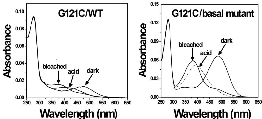
Figure 3. Analysis of UV-vis spectra of cysteine mutants G121C/WT and G121C/Basal mutant. Mutants were purified from COS-1 cells after regeneration with 25 \mu\text{M} 11-cis-retinal. UV-vis spectra were recorded in the dark, after acidification, and after illuminating the samples for 30 sec at 20°C.
