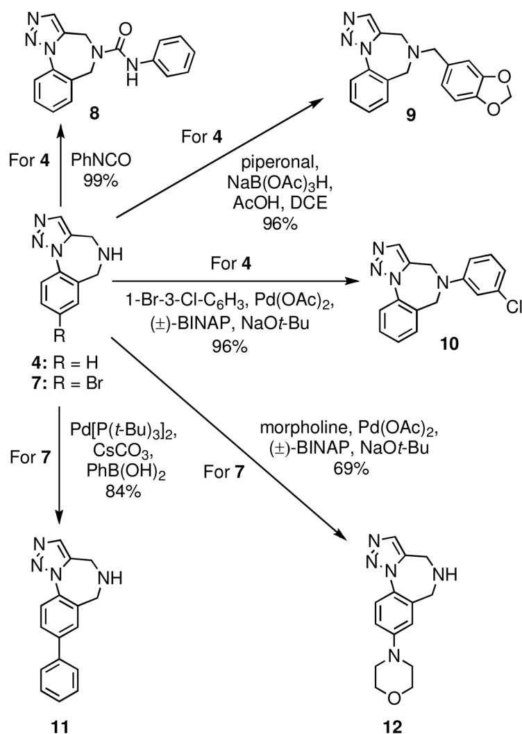
Scheme 2. Diversification of scaffolds 4 and 7
