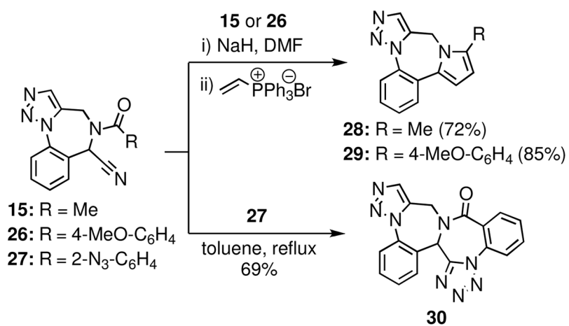
Scheme 6. Preparation of pyrole and tetrazole-fused 1,4-benzodiazepines
