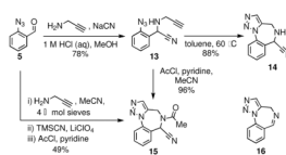
Scheme 3. Synthesis of scaffold 14 and direct access to amide 15
