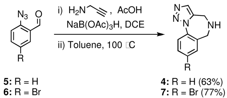
Scheme 1. Synthesis of scaffolds 4 and 7
