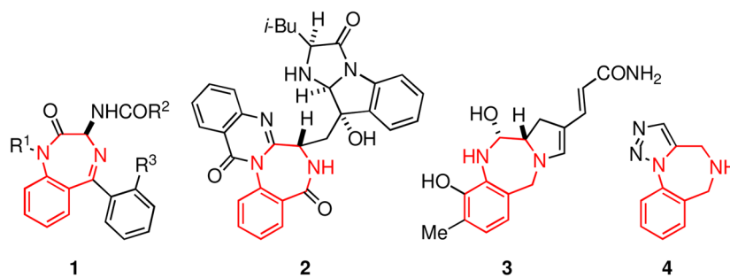
Figure 1. Derivatives of the 1,4-benzodiazepine ring system
