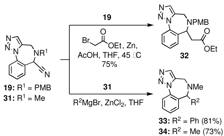
Scheme 7. Diversification using the Bruylants reaction
