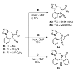
Scheme 5. Amide derived diversification of scaffold 14
