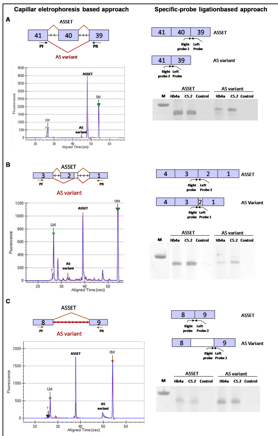
Figure 6 The influence of ERBB2-mediated expression on the regulation of AS variants. In the left panel, a schema of the microfluidic capillary electrophoresis approach is shown. The exons are represented by numbered squares according to the exons involved in the AS events for each gene. The black arrows represent the primers used for PCR amplification (PF - forward primer; PR - reverse primer). The electropherogram represents the amplification of the AS variants for the Hb4a cell line (blue line) and for the C5.2 cell line (red line). The green arrows indicates internal markers: LM (lower marker) and UM (upper marker). In the right panel, the probe-ligation approach is shown. Each pair of probe is shown for each AS variant separately, with the corresponding PCR products on 8% acrylamide gel. M - 100 bp ladder. A - gene, B - FLNA and C - TRIP6 .
