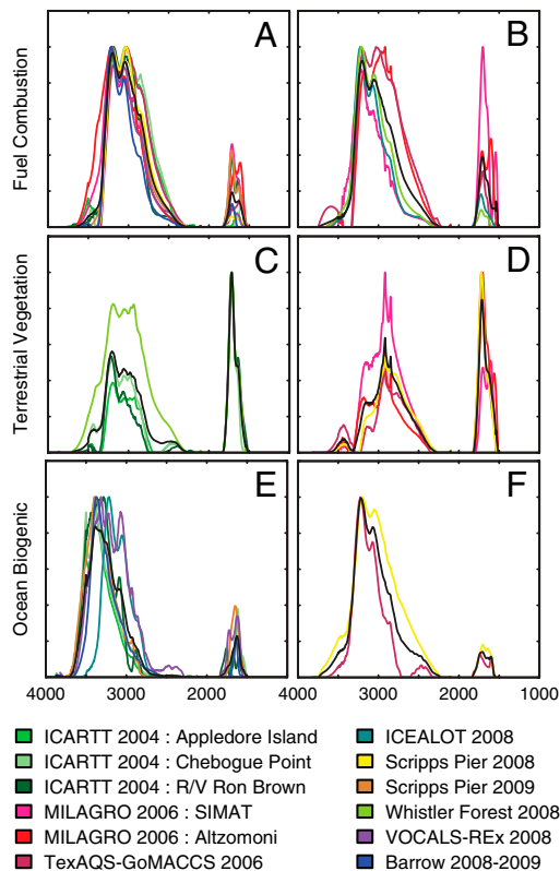
Fig. 2. FTIR spectra of PMF-based factors for fuel combustion (A, \text{O}/\text{C} < 0.4 ; B, \text{O}/\text{C} > 0.4 ), terrestrial vegetation (C, biogenic; D, burning), and ocean biogenic (E, \text{O}/\text{C} > 1 ; F, \text{O}/\text{C} < 1 ) sources for the projects with colors given in the legend. The y axes are normalized absorbance with arbitrary units.
