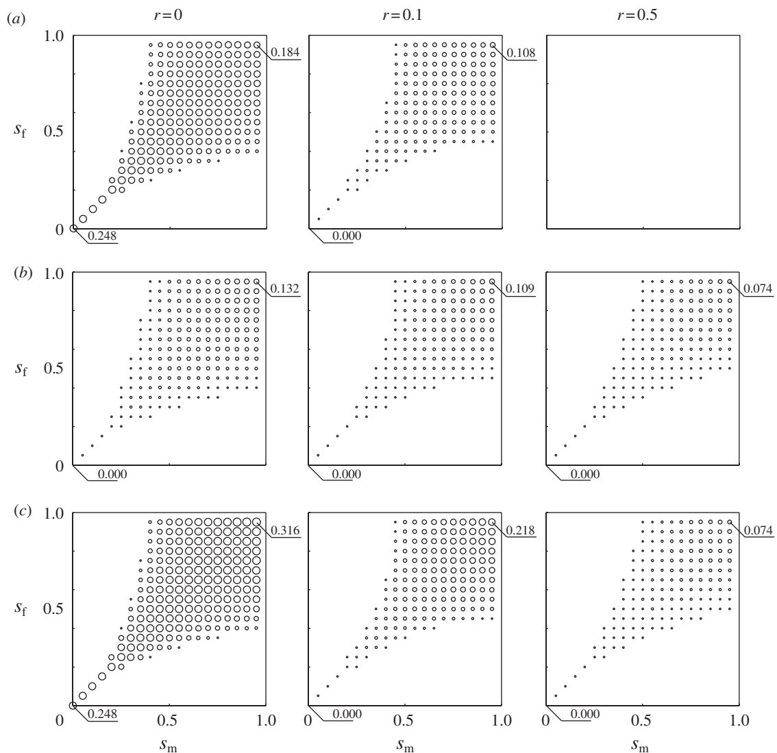
Figure 2. Linkage disequilibrium and its components for various recombination frequencies and selective strengths. LD is represented by the area of the circle at any given point ( s_m , s_f ) in the parameter space. The axes of each plot are the selection coefficient in males s_m ( x -axis) and females s_f ( y -axis). Recombination rate, r , differs for each column, increasing from left to right. (a) Average LD in gametes 1/2 (D_x + D_y) . (b) Twice covariance between allele frequencies, 2 \text{Cov}(p, q) . (c) Total LD, D_T , in zygotes.
