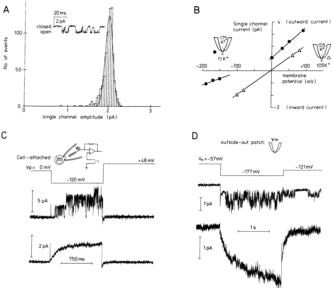
FIG. 3. Currents through individual K^+ -selective channels: Amplitude distribution (A), current-to-voltage relationship (B), and averaged time courses of outward (C) and inward (D) single-channel currents in response to voltage pulses. (A) The distribution of single-channel current amplitudes (step sizes) at a membrane potential of -100 mV in an outside-out patch in symmetrical 105 mM K^+ solutions is shown. A Gaussian fit shows that the mean single-channel current was 2.0 \pm 0.1 pA. (Inset) Sample recording of bursts of single-channel openings. (B) Amplitude of single K^+ -channel currents as a function of membrane potential in two outside-out patches. Data from a patch with 175 mM K^+ ( 170 mM KCl/5 KOH ) on the cytoplasmic membrane side and 11 mM K^+ (solution I) on the outside (see Inset) ( \bullet ). The single-channel conductance of both inward and outward currents in symmetrical 105 mM K^+ solutions (solution VI) was fitted to 20.3 pS ( \Delta ). Points were obtained as shown in A. (C) Recordings of outward currents through K^+ channels and averaged current in a cell-attached membrane patch with 12 mM K^+ (solution II) in the pipette and in the bath. The potential of the membrane patch underlying the pipette ( V_m - V_p ) was depolarized (inside positive) by imposing voltage steps ( V_p = -120 mV) on the outer membrane face (see Inset). The upper current trace shows that upon depolarization ( V_p = -120 mV), discrete outward current pulses appeared, which indicated the opening of single K^+ channels. After repolarization of the membrane to V_p = +48 mV, an inward channel current can be seen. The lower trace is an average of 80 consecutive single-channel recordings obtained as in the upper trace and shows the activation and deactivation time course of single channels. (D) Recording of inward currents through K^+ -selective channels in an outside-out patch with 105 mM K^+ on the cytoplasmic membrane side and 11 mM K^+ on the outside (see Inset). The upper current trace shows that hyperpolarizing voltage steps from a membrane potential of -57 mV to a pulse potential of -177 mV elicited inward single-channel currents. When the potential was stepped back to -121 mV, channel activity decreased. The lower trace is an average of 58 consecutive current traces and shows a slowly developing inward current that deactivated upon repolarization to -121 mV.
