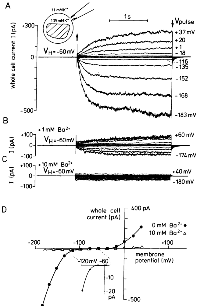
FIG. 1. (A) Recordings of K + currents in a whole guard-cell protoplast. (B and C) Partial block of K + currents by Ba 2+ ions. (D) Current-to-voltage relationship of whole-cell currents. The cytoplasm of the protoplast was loaded with 105 mM K + (solution V) via the tightly sealed pipette, while the cell was bathed in 11 mM K + (solution I) (see Inset ). (A) Superposition of consecutive recordings of ionic currents across the plasmalemma of a guard cell in response to individual voltage pulses of 2.5-s duration. Each voltage pulse started at the upward pointing arrow and stopped at the downward pointing arrow. The membrane potential was held at -60 mV ( V_H ) and stepped to potentials ranging from V_{Pulse} = -183 to +37 mV. Depolarizations caused outward currents (upward deflections), and hyperpolarizations produced inward currents seen as downward deflecting traces. (B and C) Both inward and outward currents were partially reduced by addition of 1 mM BaCl 2 (B) and 10 mM BaCl 2 (C) to the bathing solution. (D) Whole-cell current plotted before (●) and after (△) addition of 10 mM Ba 2+ as a function of membrane potential during the voltage pulse. ( Inset ) Magnification of the plot between -60 and -120 mV in solutions without Ba 2+ .
