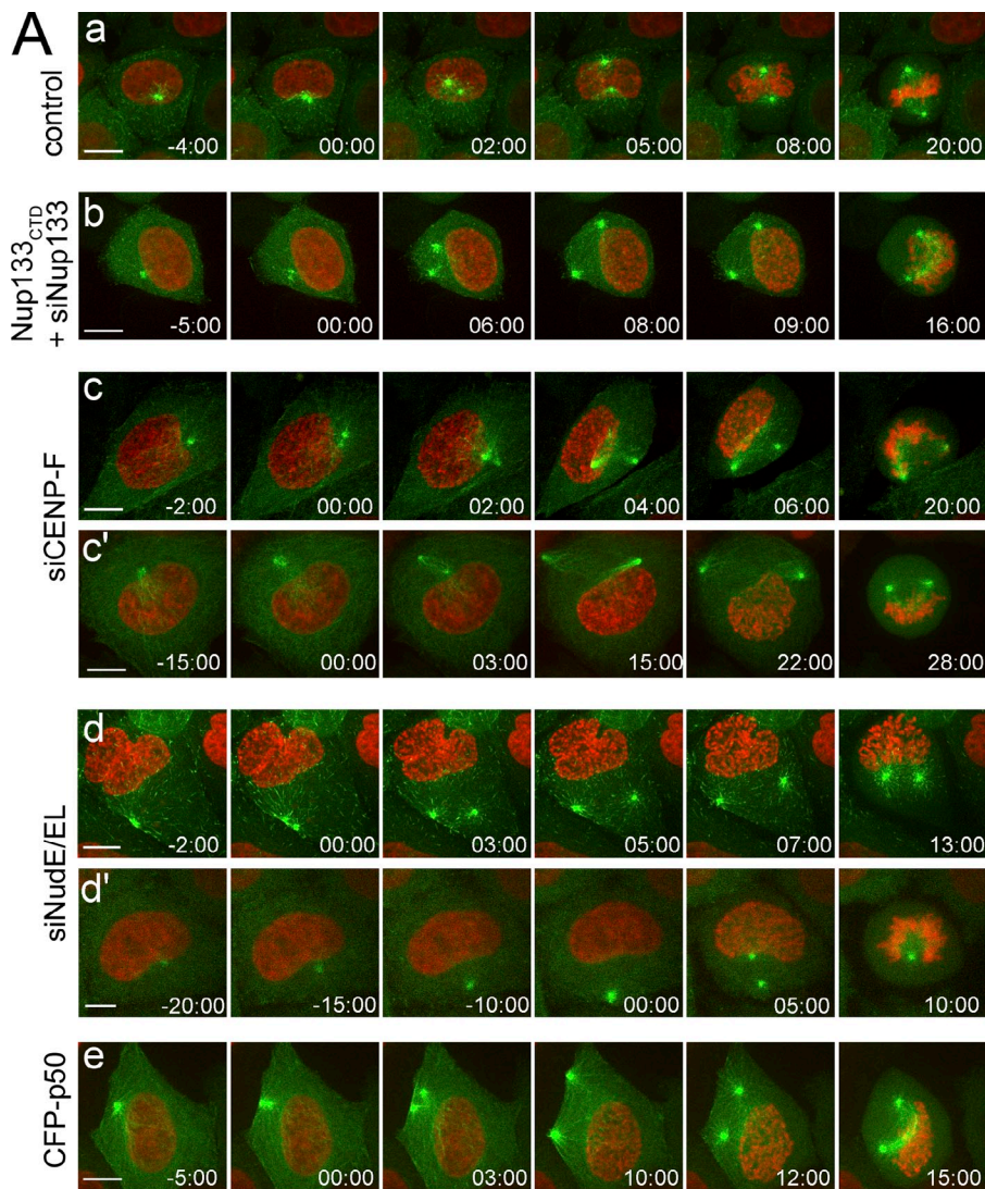
Figure 5. Interfering with Nup133-anchored dynein/dynactin impairs the tethering of centrosomes to the NE. (A) Time-lapse imaging of HeLa cells expressing EB3-GFP (green) and H2B-mCherry (red) and transfected with CENP-F (c and c'), NudE/EL siRNA duplexes (d and d'), or with a CFP-p50/dynamitin construct (e), or of cells stably expressing GFP-hNup133 CTD treated with hNup133 siRNAs and subsequently transfected with plasmids encoding EB3-GFP and H2B-mCherry (b). Time (in min:sec) was set at 0:00 when centrosome splitting just became detectable. Bars, 10 μm. See also Videos 1–6. (B) Tracks representing centrosome (CTR) movements in a control and a CENP-F-depleted cell (see Aa, Ac', and Videos 1 and 4). Trajectories before centrosome separation (red) and tracks of the separated centrosomes (blue and green) were superimposed on a schematic representation of the cell border and nuclear position (gray shading) at the beginning of the video. White and black dots indicate the positions of centrosomes at the beginning and at the end of the videos, respectively. (C) Analysis of the centrosome–NE distance over time in HeLa cells expressing EB3-GFP and H2B-mCherry and treated with scramble or CENP-F siRNA duplexes. For each cell entering mitosis, the maximum distance between the centrosomes and the NE reached during the G2/M transition was plotted over the time centrosomes spent >3 μm away from the NE. Each dot represents a single cell. The number of cell quantified is indicated.
