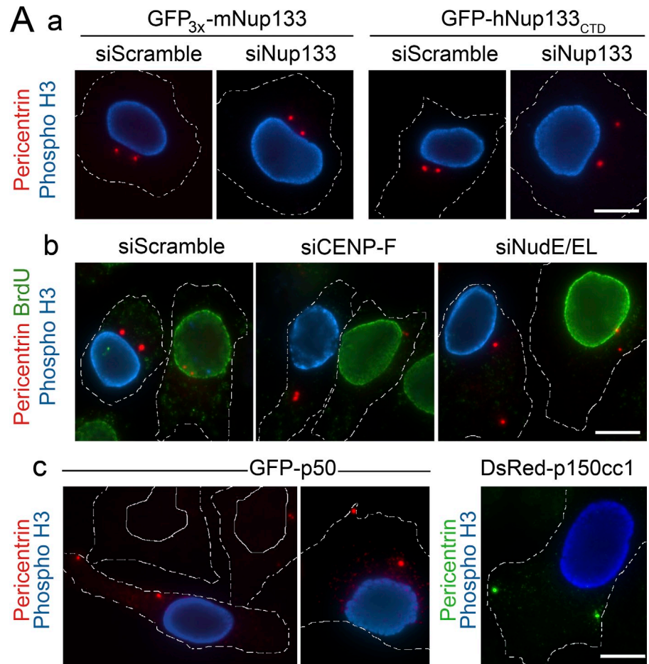
Figure 6. The Nup133-anchored network tethers centrosomes to the NPCs specifically in prophase. (A) GFP 3x -mNup133 or GFP-hNup133 CTD cells treated for 3 d with scramble or hNup133 siRNAs (a), HeLa cells treated for 2 d with scramble, CENP-F, or NudE/EL siRNA duplexes (b), or HeLa cells transfected with a GFP-p50/dynamitin or a DsRed-p150cc1 construct (c) were processed for immunofluorescence using anti-pericentriolar and anti-phospho-H3 antibodies. In b, cells were incubated before fixation with 40 \mu M BrdU for 3 h and anti-BrdU antibodies were further used. Bars, 10 \mu m. (B) Distances between centrosomes and the NE were measured on cells processed as in A. Prophase cells were identified by phospho-H3 staining and S/early G2 cells as BrdU-positive cells after a 3-h pulse with BrdU (G1 cells were not analyzed because centrosomes were reported to be very mobile at that stage of the cell cycle; Piel et al., 2000). Distances are represented as box-plots using KaleidaGraph (see Materials and methods). The black and red bars indicate the median and mean values, respectively. The total number of cells quantified is indicated (n). ***, P < 10^{-5} ; **, P < 10^{-3} ; ns, P > 0.1 obtained using the Student's t test.
