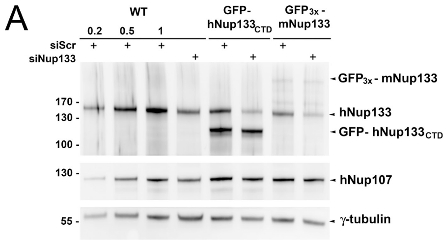
Figure 1. The N-terminal domain of hNup133 is largely dispensable for NPC assembly. (A) Control HeLa cells (WT) or cell lines stably expressing GFP-hNup133 CTD or GFP 3x -mNup133 were transfected with a scramble siRNA or with a hNup133 siRNA that does not target hNup133 CTD and only mildly impacts mNup133 expression. After 3 d, whole-cell extracts were analyzed by Western blot using anti-hNup133 (which also recognizes mouse Nup133, albeit less efficiently than human Nup133) or anti-hNup107 antibodies. Anti- \gamma -tubulin was used as loading control. To allow quantifications, decreasing amounts of the reference sample were loaded (0.2-, 0.5-, and 1-fold equivalent). (B) Cells transfected with siRNAs as in A were fixed after 3 d and processed for immunofluorescence using anti-Nup107 and mAb414 antibodies. Bar, 20 \mu m.
