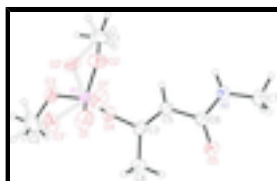
Fig. 1. The molecular structure of the title compound with the atom numbering scheme: the major part is drawn with solid lines, the minor one with open lines. Displacement ellipsoids are drawn at the 50% probability level. H atoms are presented as a small spheres of arbitrary radii.
