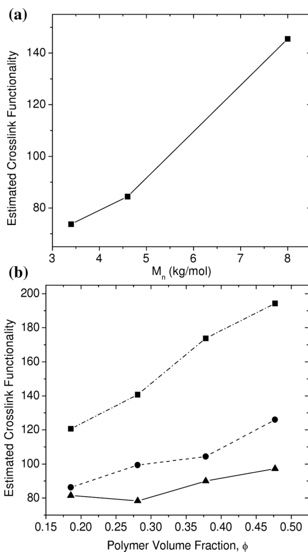
Figure 8. (a) Estimated crosslink functionalities as a function of M_n for UV-polymerized PEG-DA-50% hydrogels swollen to equilibrium. (b) Estimated crosslink functionalities for networks polymerized in situ by the SAXS x-ray radiation for PEG-DA(3.4k) ( -\blacktriangle-\blacktriangle- ), PEG-DA(4.6k) ( --\bullet--\bullet-- ), and PEG-DA(8.0k) ( ---\blacksquare---\blacksquare--- ).
