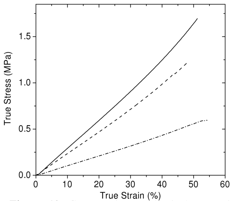
Figure 10. Compressive mechanical properties for equilibrium-swollen PEG-DA(3.4k) (—), PEG-DA(4.6k) (----), and PEG-DA(8.0k) (-·-·-) hydrogels that were prepared at 50% wt/wt.
