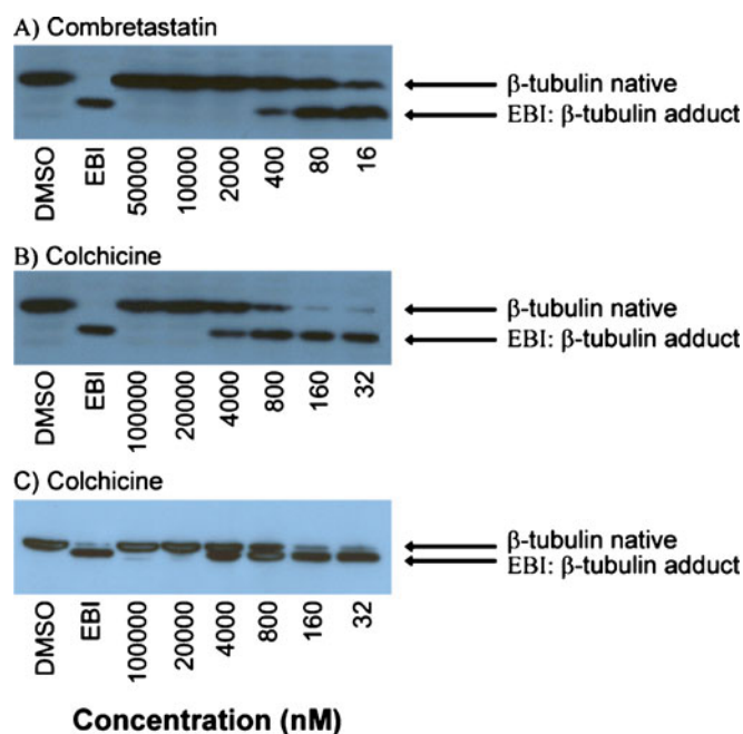
Fig. 1 Effect of escalating concentrations of combretastatin A-4 and colchicine on the inhibition of the bithioalkylation of Cys-239 and Cys-354 of \beta -tubulin by N,N' -ethylene-bis(iodoacetamide) on MDA-
