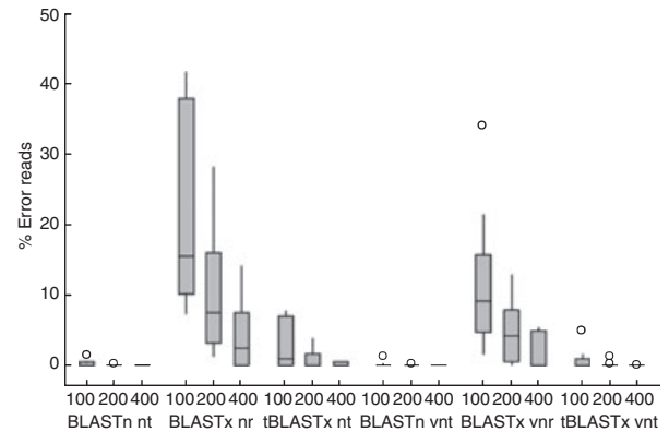
Figure 1 Box plot of total classification errors for ten human viruses according to read length and annotation method. Total errors include both ambiguous and missing identifications. Groupings are by the read length (100, 200, 400 nt), the BLAST search program (BLASTn, BLASTx, tBLASTx), and the database where 'nt' represents nucleotide database, 'nr' represents amino acid database, and 'v' represents virus only database. In each box the centreline represents the median, the top and bottom of the box represent the 25th and 75th error percentiles, and the lines represent the data spread. Outliers, marked by circles, were outside three standard deviations of the median. Outliers for Rotavirus were >80% error for the BLASTx nr and tBLASTx nt cases and were excluded from the graph. Complete results for each individual virus are listed in Table S2.
