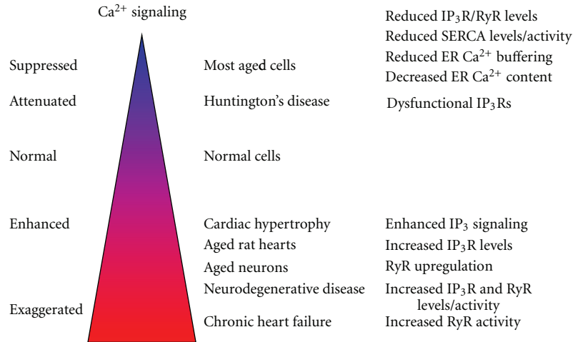
FIGURE 2: Altered Ca 2+ signaling during aging and in age-related diseases. The Ca 2+ dyshomeostasis during age is dependent on the cell type and the context. Most aged cells display decreased ER Ca 2+ content and release, due to declined IP 3 R or RyR levels, reduced SERCA activity, and decreased Ca 2+ buffering by intraluminal Ca 2+ -binding chaperones. However, in neurons and rat hearts, an enhanced Ca 2+ signaling is found, caused by increasing IP 3 R or RyR activity. Age-related diseases (neurodegeneration, cardiac hypertrophy, and chronic heart failure) are also characterized by enhanced Ca 2+ signaling. However, this property may be disease dependent, since a mouse model for Huntington's disease displayed attenuated IP 3 R1 activity due to impaired binding of Grp78 to IP 3 R1. Hence, caution should be taken with general claims.
