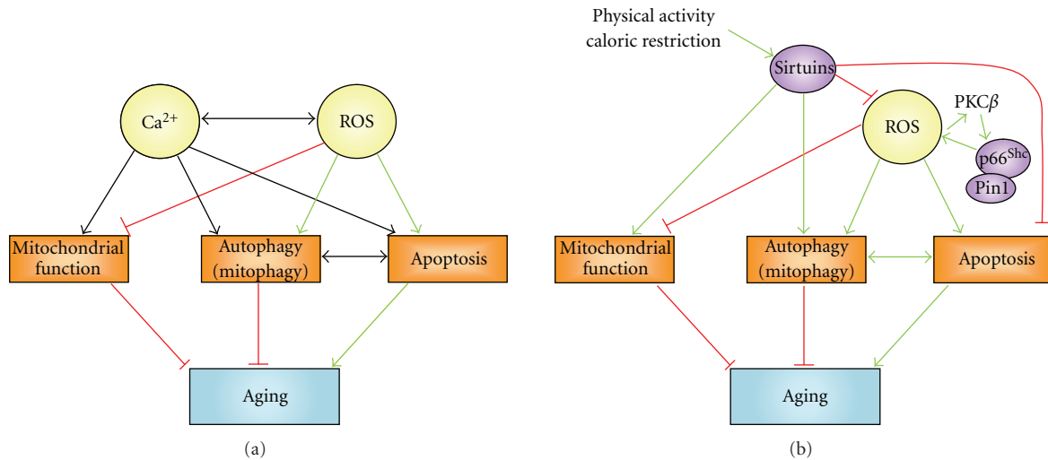
FIGURE 5: Network of interactions between sirtuins, p66 Shc , Ca 2+ , and ROS, which affect mitochondrial function, autophagy, and apoptosis, thereby controlling aging-dependent processes. (a) Ca 2+ signals may increase or prevent aging. Ca 2+ signals are characterized by different spatiotemporal characteristics and subsequently different outcomes on mitochondrial function, autophagy, and apoptosis. For example, a constitutive Ca 2+ transfer from ER to mitochondria would stimulate mitochondrial function and inhibit autophagy and apoptosis, while a mitochondrial Ca 2+ overload would be proapoptotic. The interplay between mitochondrial Ca 2+ elevations and ROS production is a critical determinant in the apoptotic outcome at the level of the mitochondria, which function as co-incidence detectors. Therefore, high mitochondrial Ca 2+ concentrations and ROS act as a double-hit mechanism, triggering mitochondrial-dependent apoptosis. (b) Sirtuins are mainly antiaging genes via the promotion of mitochondrial function and autophagy and inhibition of apoptosis. They also act inhibitingly on ROS. Sirtuin function may be enhanced by restricting caloric intake or increasing physical activity, thereby extending lifespan. Increased ROS activate the Pin1- p66 Shc complex, which, in turn, promotes the production of ROS and subsequently mitochondrial damage. Therefore, p66 Shc may help to target damaged mitochondria and activate cellular processes that deal with dysfunctional mitochondria and oxidative stress. The outcome, however, can be dual: aging may be enhanced via a complete removal of the cell through apoptosis, while the selective removal of the damaged mitochondria through mitophagy, leaving the cell with predominantly healthy mitochondria, may slow down the aging process. Green arrows: stimulation; red lines: inhibition; black arrows: stimulation or inhibition.
