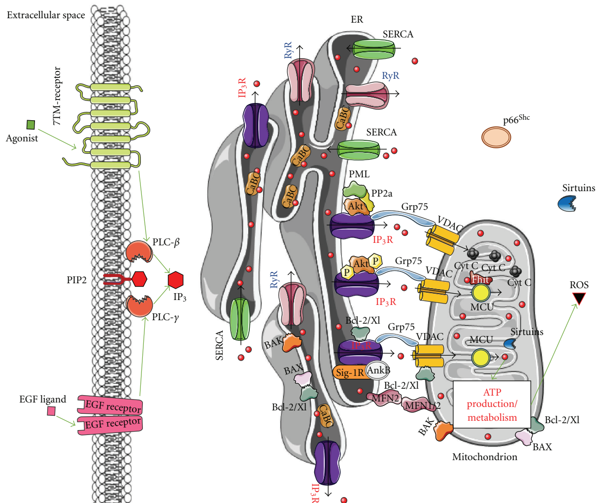
FIGURE 1: In a healthy cell, ER Ca 2+ -handling components tightly regulate mitochondrial function and bioenergetics, representing the different key players involved in intracellular Ca 2+ signalling with particular emphasis on the ER-mitochondria connections. The ER-Ca 2+ content is regulated by channels and pumps (IP 3 Rs, RyRs, SERCAs) and by Ca 2+ -binding chaperones (CaBCs). IP 3 stimulates ER Ca 2+ release and consequently the transfer of Ca 2+ (red dots) from ER to mitochondria. Mitochondrial Ca 2+ , transported via VDAC, is directly or indirectly involved in cellular energy metabolism and in the secondary production of reactive oxygen species (ROS). It is clear that IP 3 R-mediated Ca 2+ release ought to be tightly regulated to sustain mitochondrial activity and function. As a consequence, Ca 2+ -flux properties of IP 3 Rs are tightly and dynamically regulated by accessory proteins involved in cell death and survival, like Bcl-2, Bcl-XL, PKB/Akt, Sigma-1 receptor (Sig-1R)/Ankyrin B (AnkB), and the recently identified PML. It is important to note that different regulatory mechanisms occur at the IP 3 R, which may help cell survival (like Bcl-2, Bcl-XL, PKB/Akt) or help to promote cell death (like PML). The latter is essential to prevent the survival of altered, damaged, or oncogenic cells. Thus, a tight balance between both outcomes is a requisite for cellular health and homeostasis, and a dynamic switch from prosurvival to prodeath is likely essential. In this paradigm, the production of ROS might contribute to the survival of cells by efficient detection of damaged/altered mitochondria and their removal by autophagy, while preventing excessive apoptosis. In addition, controlled apoptosis is likely to be important to eliminate cells, in which the removal of altered mitochondria by autophagy is not sufficient, thereby avoiding tumor genesis. In this process, the recently identified tumor suppressor PML may play a crucial role as it promotes IP 3 R-mediated Ca 2+ transfer from the ER into the mitochondria by dephosphorylating and suppressing PKB/Akt activity through PP2A. While PKB/Akt is known to suppress IP 3 R-channel activity by phosphorylation of the IP 3 R, the recruitment of PP2A via PML at the interorganellar ER/mitochondrial complex dephosphorylates and inactivates PKB/Akt. This suppresses PKB-dependent phosphorylation of IP 3 R and thus promotes Ca 2+ release through this channel and Ca 2+ transfer into the mitochondria. At the mitochondrial level, the tumor suppressor Fhit has been shown to increase the affinity for the mitochondrial Ca 2+ uniporter (MCU), thereby enhancing the uptake of mitochondrial Ca 2+ at low and physiologically relevant levels of agonist-induced Ca 2+ signals. Green arrows: stimulation; red lines: inhibition; black arrows: Ca 2+ flux.
