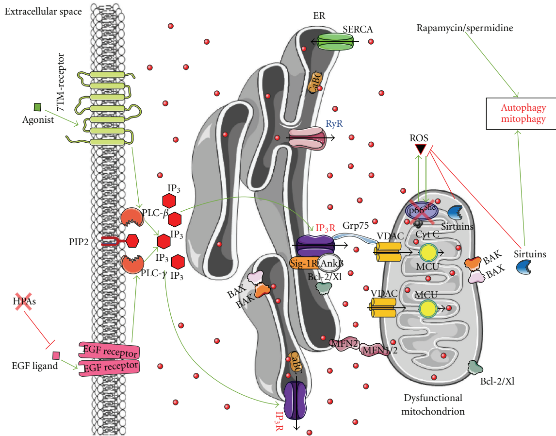
FIGURE 4: A speculative antiaging strategy based on restoring IP 3 R-mediated Ca 2+ signaling and chemical induction of autophagy. Provided the concept that aging cells are characterized by suppressed IP 3 signaling or attenuated IP 3 R, Ca 2+ -release activity is relevant in humans, and elevating IP 3 levels may compensate for the decline in the IP 3 /IP 3 R-signaling axis. This may contribute to a decline in the p66 Sbc -mediated ROS production, an activation of sirtuin-dependent mitochondrial biogenesis, and the lowering of ROS production. The final step of this compensatory response consists in the autophagic removal of the damaged mitochondria. Hence, chemical induction of autophagy (e.g., by rapamycin or spermidine) is likely critical for successful and healthy aging in human beings. It is important to note that this concept is based on a recent report on C. elegans , in which ablations of inhibitors of EGF signaling enhance IP 3 R signaling and promote healthy lifespan extension. Green arrows: stimulation; red lines: inhibition; black arrows: Ca 2+ flux.
