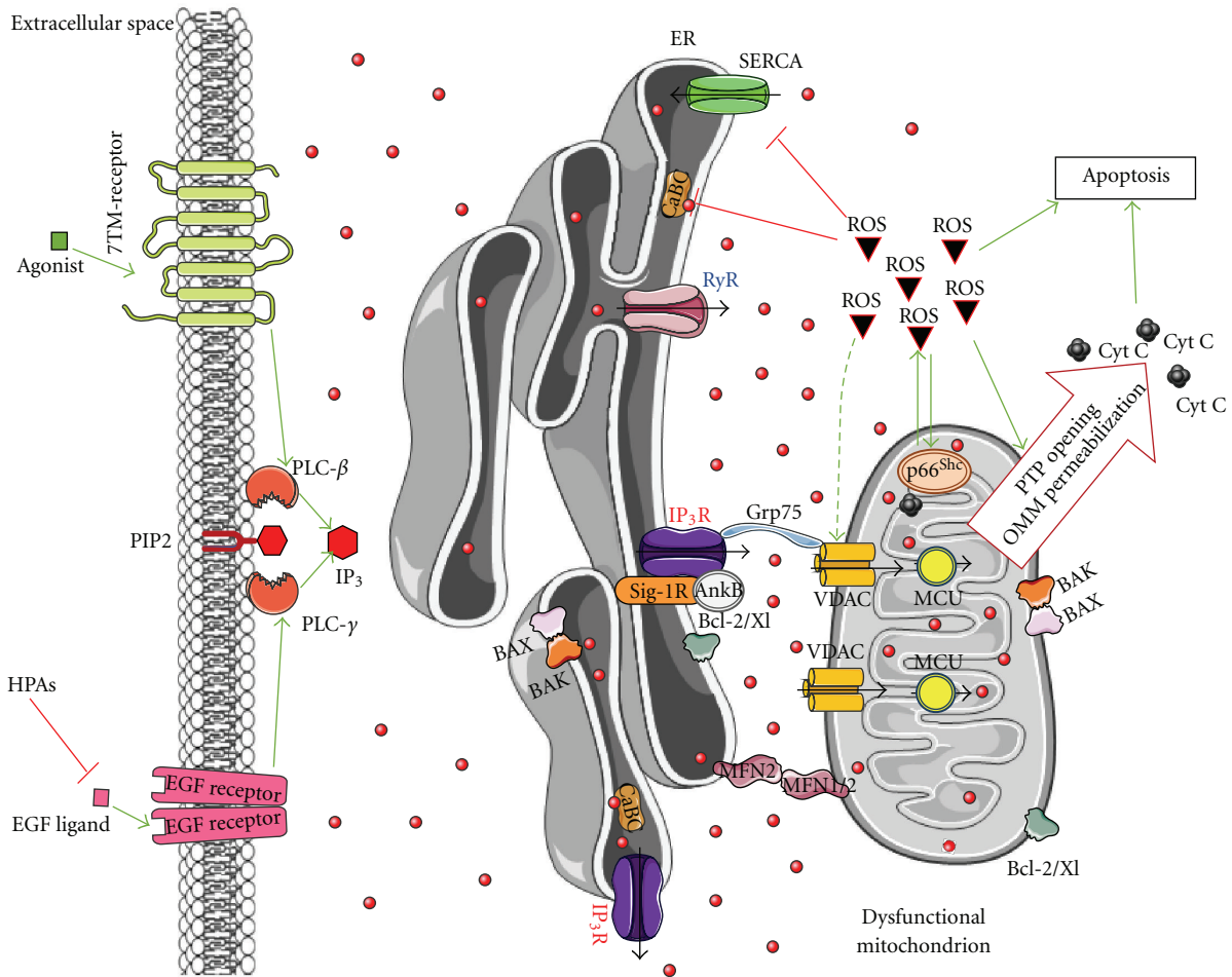
FIGURE 3: \text{Ca}^{2+} signalling and key events involved in aging. Aging cells display decreased function or expression of ER proteins ( \text{IP}_3\text{Rs} , RyRs, SERCAs, \text{Ca}^{2+} -binding chaperones (CaBC)), increased cytosolic [\text{Ca}^{2+}] , suppressed agonist-mediated signaling, and accumulation of damaged mitochondria due to declined autophagic activity. The simultaneous increase in disorganization and dysfunction of the \text{Ca}^{2+} -handling proteins and the decline in autophagy will result in the exaggerated production and excessive accumulation of ROS. These events may lead to both ER stress and mitochondrial dysfunction, like PTP opening and OMM permeabilization with the consequent release of apoptogenic factors and cell death. \text{p66}^{\text{Shc}} and sirtuins take part in this scenario. \text{P66}^{\text{Shc}} translocates to mitochondria upon oxidative-stress-induced \text{PKC}\beta phosphorylation and peptidylprolyl isomerization by Pin1, thereby supporting ROS production. Sirtuins are downregulated and unable to exert its antiaging effect. It is important to note that while \text{p66}^{\text{Shc}} ablation leads to lifespan extension, high levels of \text{p66}^{\text{Shc}} have been observed in centenarians. While in normal cells, ROS help to detect and remove altered mitochondria through autophagy, thereby maintaining cellular health, the excessive release of ROS in combination with the decline in autophagy observed during aging may underpin the age-related cell-death processes. In this respect, the recently identified inhibitors of EGF-receptor signaling, the high-performance advanced age phenotype proteins (HPA-1 and HPA-2), whose knockdown promotes locomotory health span of C. elegans , may point towards an important role of proper agonist-induced \text{Ca}^{2+} signaling via the \text{IP}_3\text{R} axis. The relevance of these ligands or of attenuated agonist-induced signaling in humans needs to be established. However, recent evidence indicates that dysfunction of \text{IP}_3\text{Rs} during ER stress promotes cell death and underlies a neurodegenerative disease, like Huntington's disease. Given the central role of proper \text{IP}_3\text{R} function for mitochondrial bioenergetics and ATP production, the decline of \text{IP}_3\text{R} activity observed during ER stress or attenuated upstream signaling linked to \text{IP}_3 may be very relevant for age-related apoptosis but require further investigation. Green arrows: stimulation; red lines: inhibition; black arrows: \text{Ca}^{2+} flux; dashed-green arrow: stimulation/damage.
