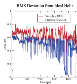
Figure 2. Comparison of the RMSD of the helix during the folding trajectory at 298 K for the 7-replica HAREM and the 64-replica normal REM.
