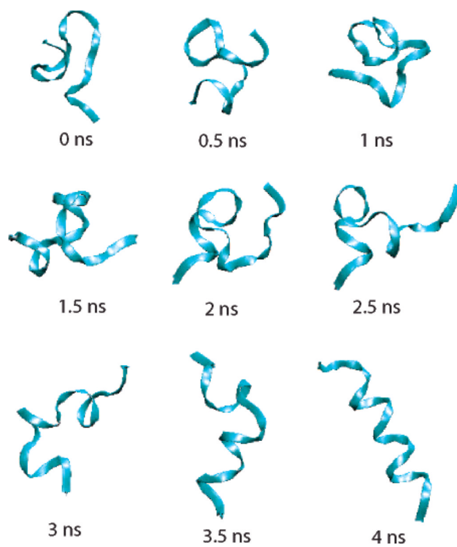
Figure 4. Snapshots of the peptide in one replica during the folding process.
