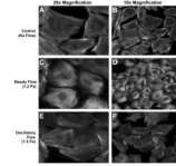
Fig. 1. Change in F-actin organization of MC3T3-E1 osteoblastic cells in response to no flow control ( A and B ), unidirectional steady flow ( C and D ), and oscillatory flow ( E and F ) for 1 h. Only application of steady unidirectional flow ( C and D ) resulted in the reorganization of the actin cytoskeleton into distinct stress fibers.
