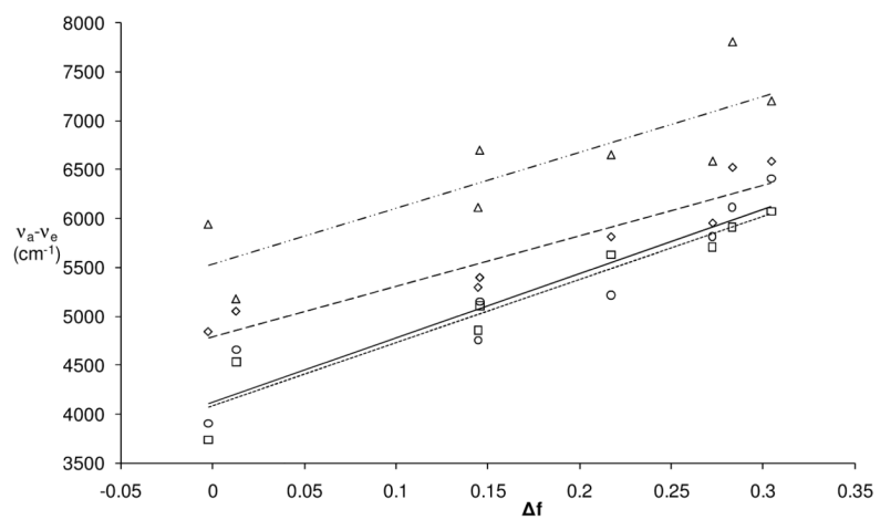
Figure 2. Lippert-Mataga plots for 7 ( \Delta , -·-·-), 8 ( \diamond , - - -), 3 ( \square , ····) and 1 ( \circ , ———).
