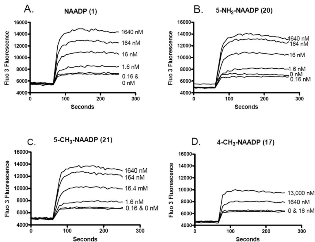
Figure 1. Fluorimetric calcium release traces from sea urchin egg homogenates induced by the addition of increasing concentrations of NAADP and three selected NAADP analogs. Calcium-ion concentration was measured fluorimetrically using the calcium sensitive dye Fluo-3. The effect of the addition of increasing concentrations of NAADP ( 1 )(A), 5-NH 2 -NAADP ( 20 )(B), 5-CH 3 -NAADP ( 21 )(C), and 4-CH 3 -NAADP ( 17 )(D) on fluorescence are shown.
