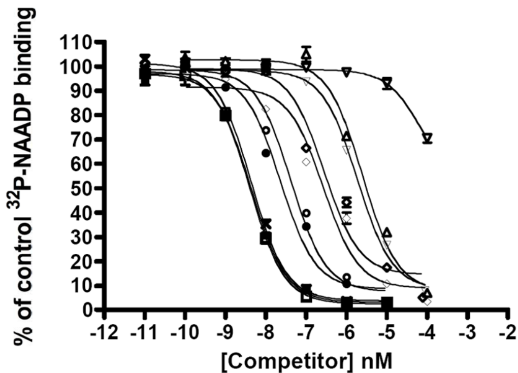
Figure 4. Competition radioligand binding curves for NAADP (1)(■) and the nine analogs (16-24) in sea urchin egg homogenates: 5-NH 3 -NAADP (20)(□), 5-CH 3 -NAADP (21)(×), 5-CH 2 CH 3 -NAADP (23)(●), 5-N 3 -NAADP (24)(○), 4-NH 3 -NAADP (16)(◇), 4-CH 3 -NAADP (17)(◊), 4- n -butyl-NAADP (18)(▽), 4-phenyl-NAADP (19)(△), and 5-CO 2 H-NAADP (22)(∇). Each plotted point represents the mean of a minimum of three determinations.
