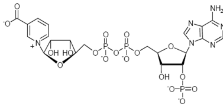
Nicotinic Acid Adenine Dinucleotide Phosphate (NAADP), 1
