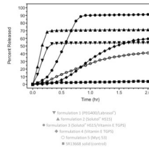
Figure 1. Release of SR13668 from the reference formulation and four self-emulsifying formulations in hard gelatin capsules, as a function of time using USP dissolution unit 2 at 37°C with paddles at 50 rpm and 900mL water as the dissolution medium.
