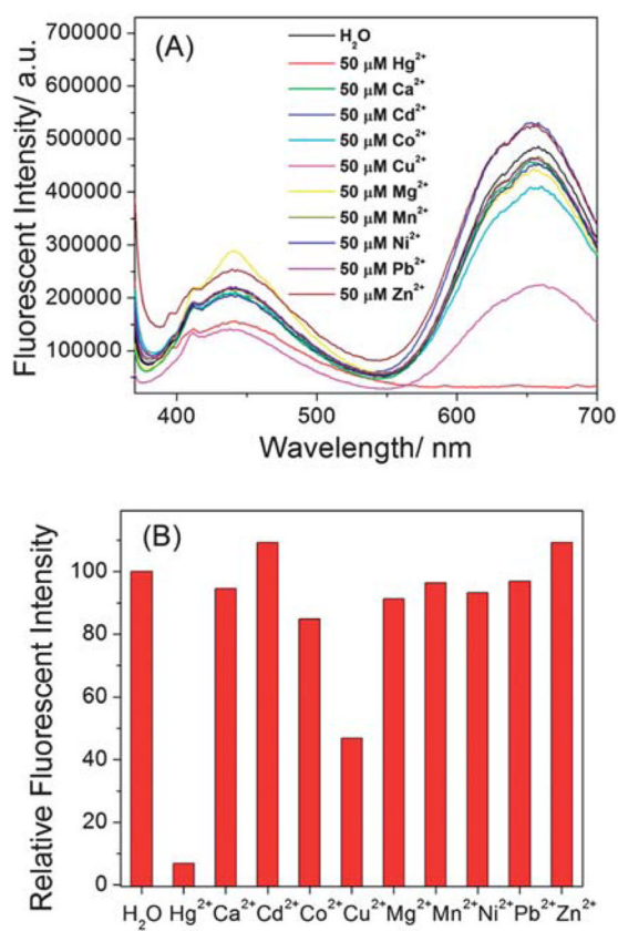
Fig. 7. (A) The fluorescent spectra of 10% diluted probes LsGFC (~ 3.4 μM) in the absence and presence of 50 μM different metal ions, (B) the relative fluorescent intensity at 657 nm vs. metal ions. The excitation wavelength was 360 nm.
