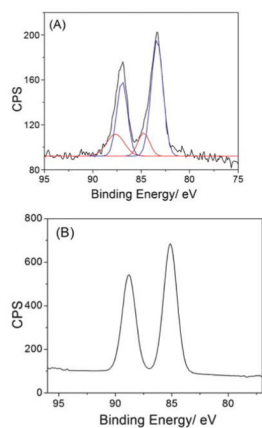
Fig. 4. XPS spectra of Au 4f of the as-prepared LsGFC (A) and lysozyme-HAuCl 4 complex alone (B) deposited on the silica wafer. In panel (A), the original spectrum is in black, the Au + 4f spectrum after analysis is in red, and the Au 0 4f spectrum after analysis is in blue.
