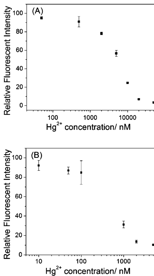
Fig. 6. The relative fluorescent intensity at 655 nm vs. Hg 2+ concentration by using 10% diluted LsGFC probes ( \sim 3.4 \mu\text{M} ) (A) and 1% diluted LsGFC probes ( \sim 0.34 \mu\text{M} ) (B). The excitation wavelength was 360 nm. The error bars represent the standard deviation of three measurements.
