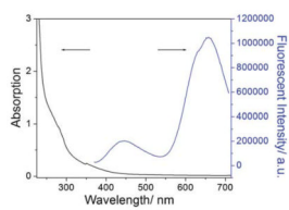
Fig. 2. Absorption (left) and fluorescent (right) spectra of the as-prepared LsGFC. The excitation wavelength was 360 nm.
