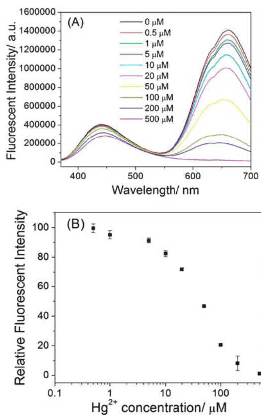
Fig. 5. (A) The fluorescent spectra of as-prepared LsGFC probes (~ 34 μM) in the absence and presence of different concentrations of Hg 2+ , (B) the relative fluorescent intensity at 660 nm vs. Hg 2+ concentration. The excitation wavelength was 360 nm. The error bars represent the standard deviation of three measurements.
