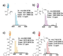
Figure 3. Detection of PacH-bound biosynthetic intermediates by FTMS after trypsin digestion. ATP, L-Phe, L-Ala, DABA, PacPH were present in all assays. PacU was present in assays b) and d), while PacDJLNO were present in assays c) and d). Theoretical mss calculations are shown in Figure S4.
