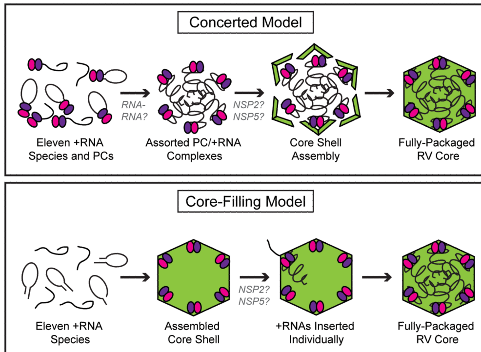
Figure 4. Models of RV +RNA assortment and packaging
