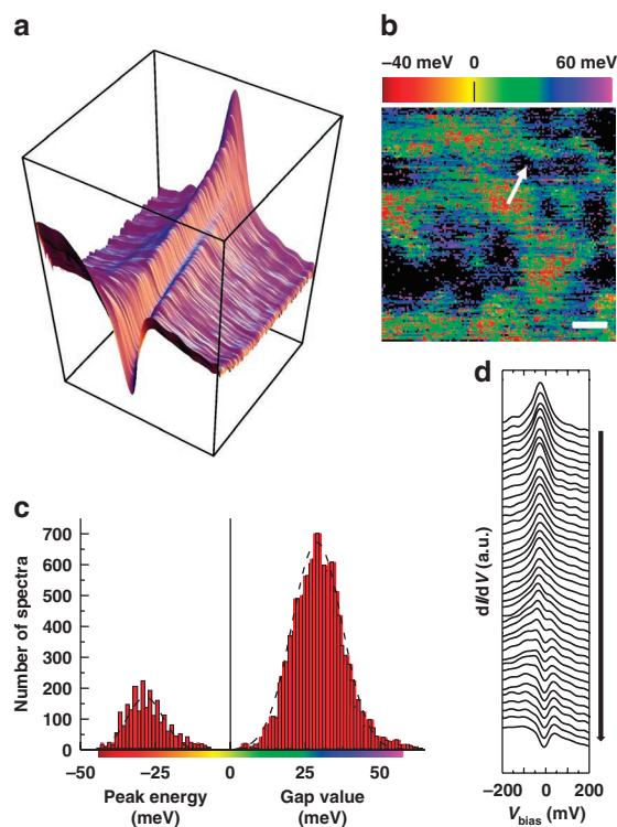
Figure 1 | Low-temperature (5 K) STS spectroscopy of as-grown Bi-2201 (AG11K). (a) Three-dimensional overview of the data: each curve is the average of 60 spectra sharing the same E_p value ( E_p is the peak position for single-peak spectra, and half the peak-to-peak distance for two-peak spectra); the curves are sorted by increasing E_p . Note the smooth transition between completely different curves at extremal values of E_p . (b) E_p map of a 14 \times 14 nm 2 area. The white bar corresponds to 2 nm. The red and yellow regions correspond to negative E_p (single-peak spectra) while in green, blue and purple regions, the spectra exhibit a gap width of \Delta_p = E_p . Red-yellow spots are surrounded by green regions where the smallest gap is measured ( \sim 20 meV). Black patches are composed of spectra ( \sim 4,000 in total) in which no gap could be extracted due to a missing left peak (or sometimes no peak at all); these spectra are not included in the histogram of panel c. (c) Distribution of E_p values. The dashed lines are Gaussian fits. The average peak position and average gap values are -28 and +29 meV, respectively. (d) Spatial evolution of the spectra on the path depicted by the arrow in b. The path goes from a red region (top-most single-peak spectrum) to a black region where the left coherence peak is barely visible. Notice the strong similarity with the global evolution shown in a.
