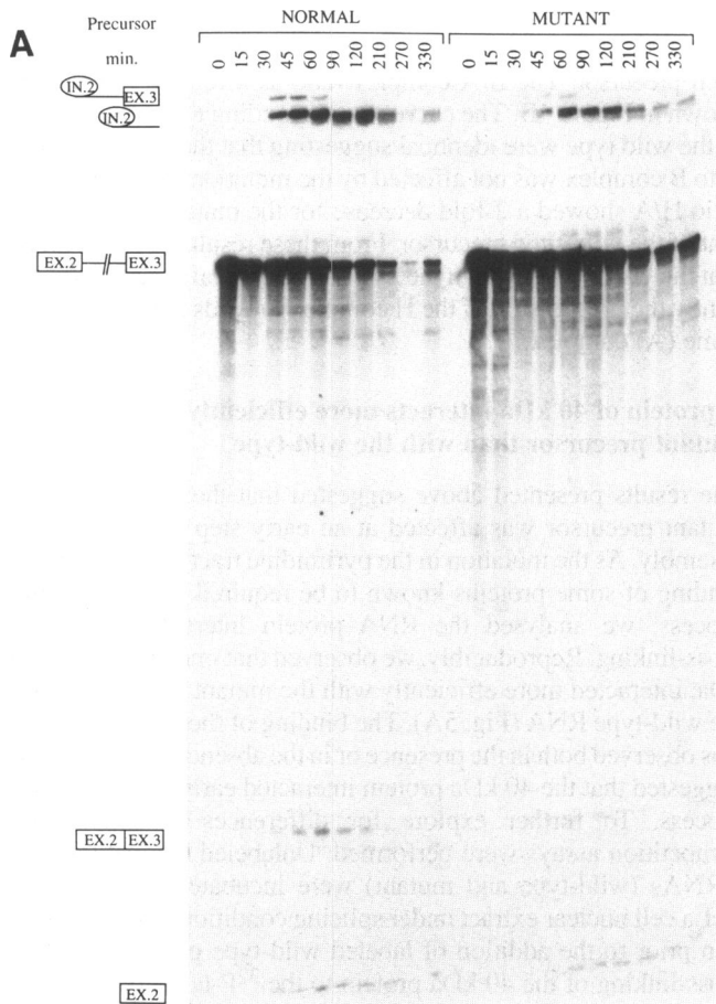
Figure 3. In vitro splicing reaction of the shorter wild-type and mutant transcripts (517 nt). Splicing was for the times indicated.
