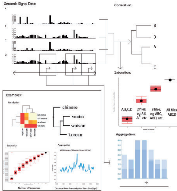
Fig. 1. Uses of ACT using signal tracks from various sources. Signal around all TSSs is aggregated to give an average signal profile, for example of Baf155 binding around TSSs (Encode Project) (aggregation). Figure made in Excel (correlation). Multiple signal tracks are correlated to show which tracks are more or less related to each other. In the selected example, a heatmap of the SNP track correlation between four individuals (dbSNP) leads to a dendrogram of their phylogenetic relationship. Figure made using Web ACT. Each additional signal track increases the number of base pairs covered (saturation). When the addition of signal tracks is considered in all possible combinations, the average increase in coverage, with error bars, can be visualized by a saturation plot. In the example, data are taken from individuals from dbSNP [with additional genomes from Ahn et al. (2009), Bentley et al. (2008), Drmanac et al. (2010), Kim et al. (2009)]. In each box plot, the top and bottom pink bars correspond to the maximum and minimum normal values, the top edge, middle line and bottom edge of the box correspond to the top 25 percentile, median and bottom 25 percentile, the black dot is the mean, and red circles are outliers. Figure made using ACT downloadable saturation program.
