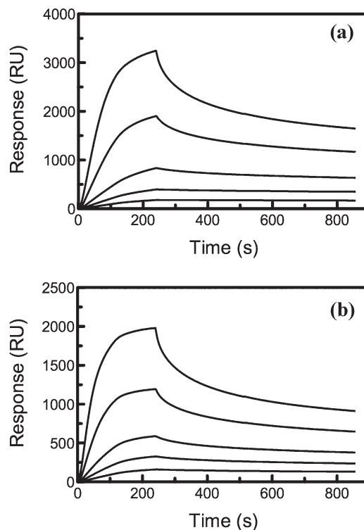
Figure 3. SPR sensorgrams for TGF \beta_1 injection over surfaces functionalized with immobilized peptides: (a) CCGKRIWFIPRSSWY and (b) CCGWSHW. TGF \beta_1 was injected at 100, 50, 20, 10, 5, and 0 nM in HBS-EP buffer at a flow rate of 50 \mu L/min. Sensorgrams represent the average signal for three injections.
