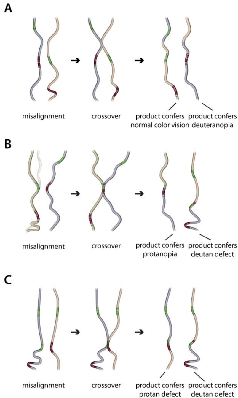
Fig.2. Recombination produces an opsin array that causes color vision deficiencies. A) Misalignment of the opsin gene arrays on the two X-chromosomes in a female allows a crossover in the region between the L and M genes in one array and the homologous region downstream of the M gene in the other array. This produces two new X-chromosome opsin gene arrays. One array has an L gene and two M genes and will confer normal color vision. The second array has a single opsin gene, an L gene, and produces the color vision defect, deuteranopia, when inherited by a male. B) Misalignment of the opsin gene arrays on the two X-chromosomes in a female allows a crossover between the L gene on one X chromosome and the M gene on the other X-chromosome. This produces two new arrays
