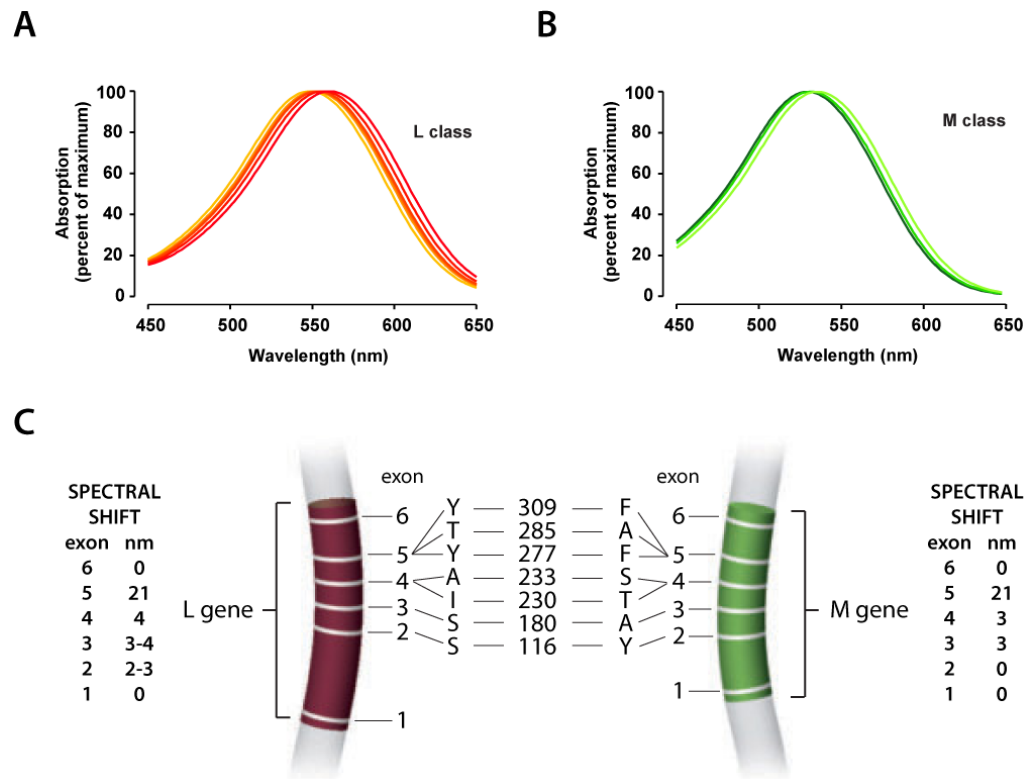
Fig.1. A) Spectral tuning of human L and M cone photopigments. A) L-class pigments absorb maximally near 560 nm. B) M-class pigments absorb maximally near 530 nm. C) Genes encoding the L and M opsins each have 6 exons represented by narrow white bars and numbered 1 through 6. The colored regions indicate the exons in the L and M opsin genes. The genes are drawn to scale. Codons that specify amino acids involved in spectral tuning are indicated using the single letter amino acid code and the codon number/amino acid position is indicated by the numbers in the middle of the panel. The single letter amino acid code is as follows: Y = tyrosine, T=threonine, A=alanine, I=isoleucine, S=serine, F=phenylalanine. The magnitude of the spectral shift in nanometers (nm) produced by the indicated amino acid differences specified by each exon are indicated on the far right and far left.
