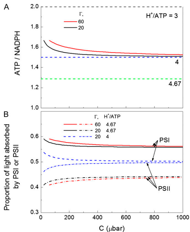
Figure 1. A, The ATP/NADPH ratio required to satisfy CO 2 assimilation and photorespiration as a function of CO 2 partial pressure at Rubisco. The ratio depends on the value assumed for \Gamma_* ( \mu\text{bar} ), the CO 2 photocompensation point, which increases with temperature. The ratios produced by linear electron flow are shown assuming three, four, and 4.67 H + /ATP. B, The proportion of light absorbed by PSI and PSII necessary to satisfy the linear electron flow and cyclic electron flow required to provide the ATP/NADPH for different values of \Gamma_* and likely H + /ATP ratios. A constant value is frequently used to calculate linear electron flow from chlorophyll fluorescence.
