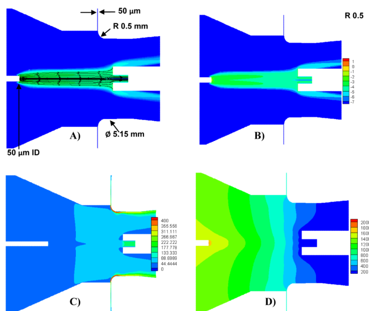
Figure 6. Results with air amplifier A) Droplet Stream lines B) Logarithm of Droplet Density C) Velocity Contours D) Electrical Potential. Focusing effect of the air amplifier is present as droplets remain centered axially. The distance between the ESI tip is 6 mm.
