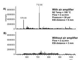
Figure 5. Spectrum comparison for 75 \mu\text{m} ESI tip, ESI flow rate of 2 \mu\text{L} and 100% water solvent composition. A) Spectrum obtained when using the air amplifier. B) Although electrospray was established, only very weak signal (below noise level) was obtained without the air amplifier. Comparing average abundance of (\text{M}+4\text{H})^{4+} and (\text{M}+5\text{H})^{5+} ions for 124 spectrum, an improvement of 34 folds is obtained using the air amplifier under these conditions.
