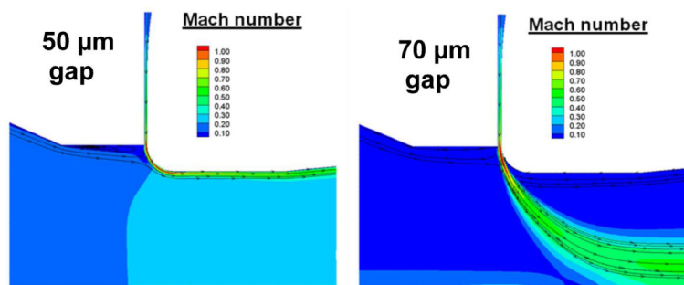
Figure 2. CFD Simulation of Coanda effect at different annular gap for a pressure of 30 PSIG. At 50 \mu\text{m} , the air jet coming from the plenum pressure curves around the Coanda surface creating a Venturi effect in the air amplifier. At 70 \mu\text{m} gap, the jet no longer stays attached to the curved surface and Coanda effect is lost.
