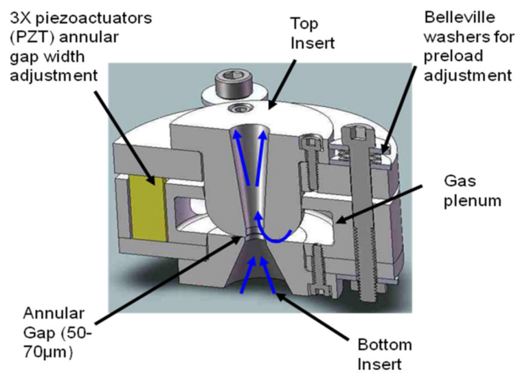
Figure 1. Section view of air amplifier assembly
