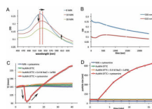
Figure 4. UV-Vis absorbance, relaxivity and particle size studies of probe stability in cysteamine and/or 0.4 M NaCl and 1xPBS
