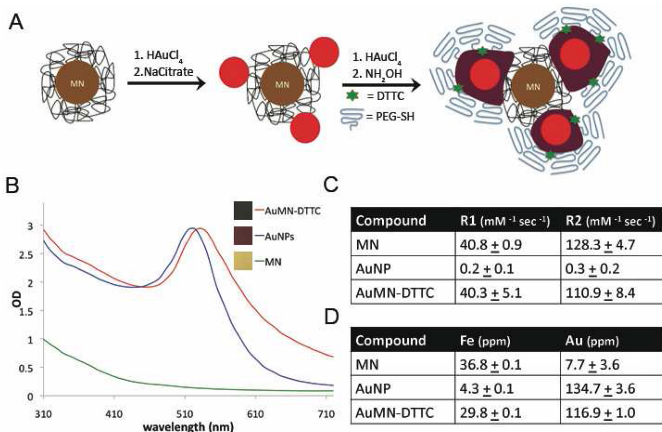
Figure 1. Synthesis and characterization of the MRI-SERS active nanomaterial (AuMN-DTTC)
