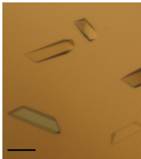
Figure 1 Single crystals of human \alpha -thrombin belonging to the orthorhombic space group P2_12_12_1 . The scale bar is 100 \mu\text{m} in length.
