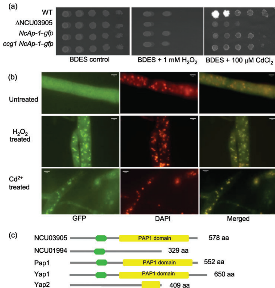
Fig. 2. Complementation of \Delta NcAp-1 and localization of NcAp-1-GFP. (a) Comparison of the phenotype of the WT (FGSC 2489), the NcAp-1 mutant ( \Delta NCU03905 ) and \Delta NcAp-1 complemented strains ( NcAp-1-gfp and ccg1 NcAp-1-gfp ) exposed to 1 mM H_2O_2 or 100 \mu M Cd^{2+} using a dilution series of conidial suspensions (from left to right: 10^5 , 10^4 , 10^3 , 10^2 , 10^1 ). Plates were incubated at 25 °C for 2 days and then evaluated for growth. (b) NcAp-1-GFP localization in a \Delta NcAp-1 ( his-3::NcAp-1-gfp ) strain grown on minimal medium (untreated, upper panels), after treatment with 30 mM H_2O_2 ( H_2O_2 treated, centre panels) or 10 mM CdCl_2 ( Cd^{2+} treated, lower panels). The left-hand panels show GFP fluorescence (NcAp-1-GFP), while the centre panels show nuclear 4,6-diamidino-2-phenylindole (DAPI) staining. The right-hand panels show merged GFP and DAPI images. (c) Domain prediction of Yap1, Yap2, Pap1, NCU03905 (NcAp-1) and its closest paralogue NCU01994. Green, bZIP motif; yellow, PAP1 domain.
