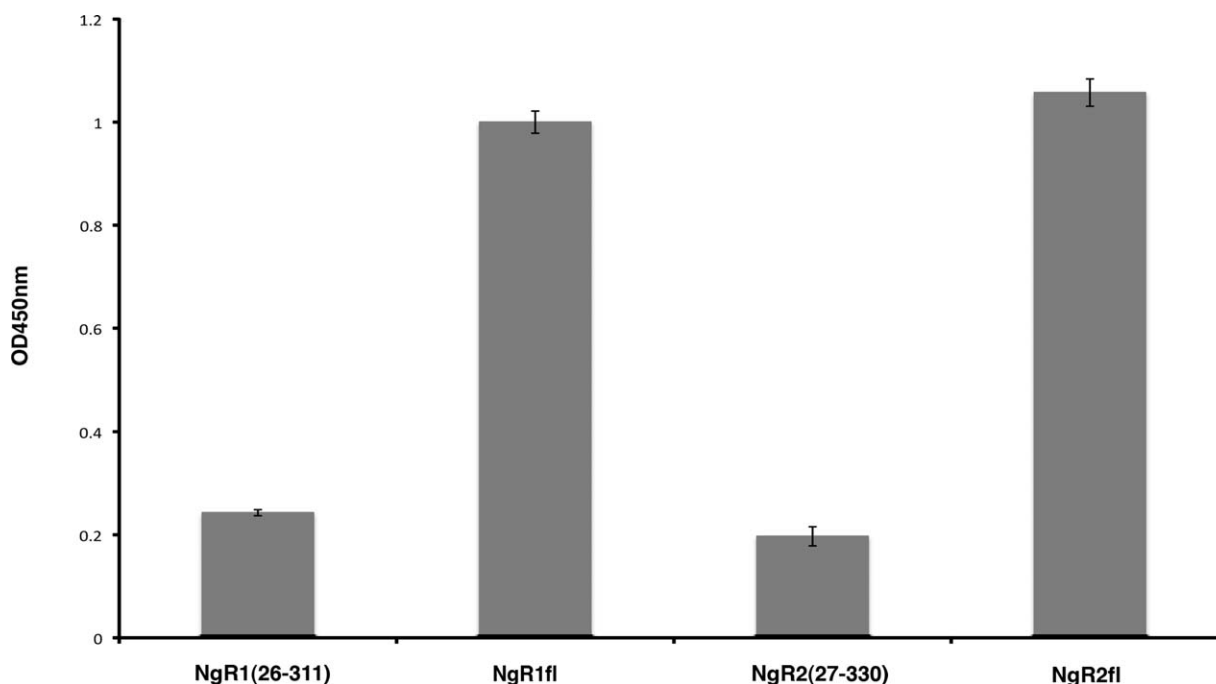
Figure 3. Comparison of the MAG binding affinities of the isolated LRR domains with that of the full-length NgR1 and NgR2 proteins. Data were corrected for Fc fragment binding to immobilized MAG and normalized with respect to full-length NgR1. Error bars represent the s.d. of four independent measurements and “fl” refers to full-length.
