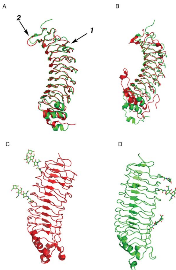
Figure 1. Structure of NgR2. (A) Comparison of the structure of NgR1-311 (red) and NgR2-310 (green). Arrows point to the differences between NgR1 and NgR2. (B) Superposition of NgR2 (330) (green) and Gplb \alpha (red). (C) Structure of NgR1 (311) with Asn-linked glycosylation shown as bonds. (D) Structure of NgR2-330 with Asn-linked glycosylation shown as bonds. Molecules in (C) and (D) are in similar orientation.
