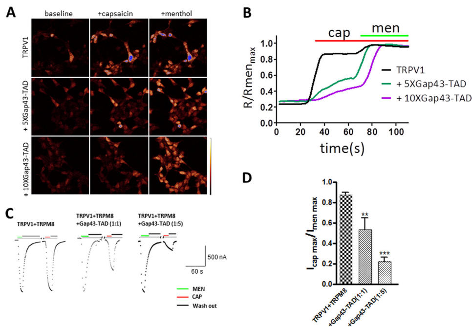
FIGURE 6. Dominant-negative effect of membrane-tethered TAD on TRPV1 channel function. A , calcium imaging of HEK293T cells co-transfected with TRPV1, TRPM8, and Gap43-tagged TAD with mole ratios of 1:1:5 or 1:1:10 (indicated as 5X or 10X), and then subjected to channel activation by 150 nM capsaicin and subsequent 500 \mu M menthol. B , normalized calcium imaging traces of TRPV1 (black) and TRPV1 + 5X (green) or 10X Gap43-TAD (purple traces) from the transfected HEK293T cells corresponding to A ; each trace is an average of 19–43 cells. Applications of capsaicin (cap, 150 nM) and menthol (men, 500 \mu M) are indicated as green and red lines, respectively. C , representative current traces recorded from Xenopus oocytes coexpressing TRPV1 and TRPM8 with Gap43-TAD at mole ratios of 1:1:1 or 1:1:5. Applications of menthol (500 \mu M) and capsaicin (250 nM) are shown in green and red bars, respectively. Gray lines indicate the zero-current. D , current amplitude comparison of maximal capsaicin-induced currents normalized to maximal menthol-induced currents from C , showing the effect of increasing ratios of Gap43-TAD on TRPV1 ( n = 5 –9 cells). Statistical significance is indicated as asterisks, **, p < 0.005 ; ***, p < 0.001 .
