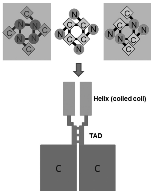
FIGURE 8. A molecular model for tetrameric assembly of TRPV channels. Top panel , an illustration of three possibilities of homotetrameric assembly mediated by N termini ( left ), C termini ( middle ), and N termini ( right ). Our findings favor that the C terminus mediates the homotetrameric assembly of TRPV1–4 channels ( middle ), not the two framed. Bottom panel shows the proposed model of tetramerization mediated by the TAD connecting the coiled-coil domain and the C termini. For clarity, only two of the four subunits are shown.
