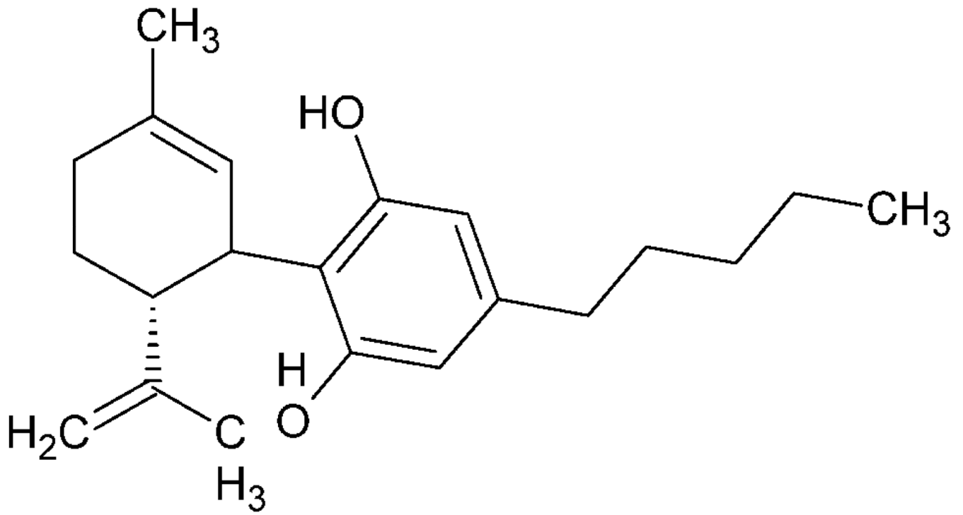
Figure 1. Chemical structure of cannabidiol (CBD).
