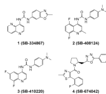
Figure 1. Structures of SB334867 and other OX1 selective antagonists.
