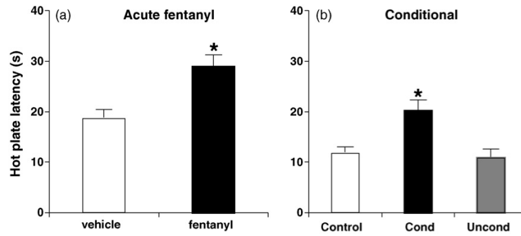
Fig. 5. Acute and conditional analgesia. (a) Acute fentanyl-induced analgesia on the 52.5 °C hot plate (0.2 mg/kg, i.p.). “*” = Significantly different from vehicle ( p < 0.05 ). (b) Conditional analgesia on the 52.5 °C hot plate. “*” = Conditioned mice (Cond) significantly different from Control and Unconditioned mice (Uncond; p < 0.05 ). Data are presented as the mean \pm S.E.M.
