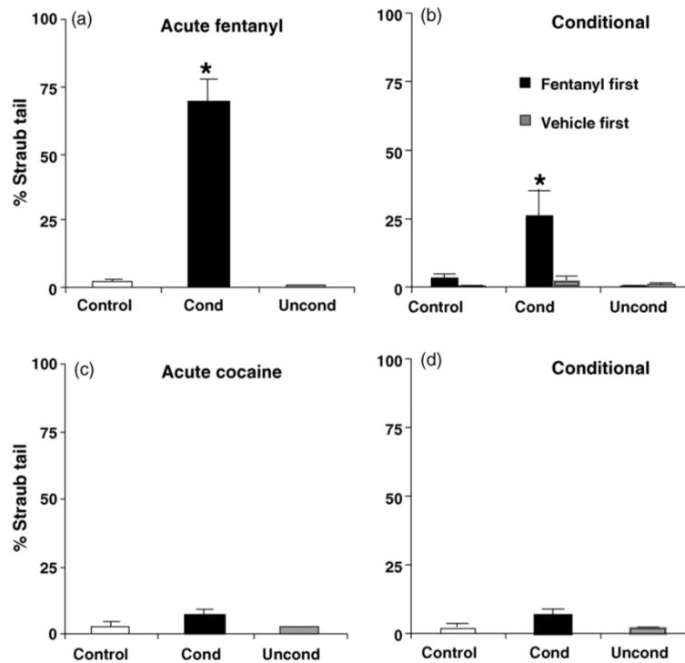
Fig. 4. Acute and conditional Straub tail. (a) Acute fentanyl-induced Straub tail (0.2 mg/kg, i.p.). (b) Conditional Straub tail for the first minute following a vehicle injection. Conditional Straub tail depended on whether the first training injection was fentanyl (“fentanyl first”) or vehicle (“vehicle first”). “*” = Conditioned mice (Cond) significantly different from Control and Unconditioned mice (Uncond) following “fentanyl first” conditioning ( p < 0.05 ). (c) Lack of cocaine response over 30 min (15 mg/kg, i.p.; given as the first injection in Conditioned mice; p > 0.05 ). (d) Lack of cocaine conditional response for the first minute following a vehicle injection ( p > 0.05 ). Data are presented as the mean \pm S.E.M.
