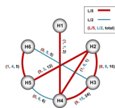
Figure 11. Helix-Helix interaction map for AgrC-I. TMHit 313 generated transmembrane (TM) helices are indicated as circles and numbered according to AgrC-I topology 37 . Interactions between the helices are indicated by the lines (or arcs). The presence of a line/arc indicates that at least one predicted atomic interaction pair exists between the helices, and the absence of a line/arc means that the program predicts no contact pairs. An interaction pair is defined as a pair of residues that have at least one pair of atoms that are separated by less than the sum of their van der Waals radii plus 0.6 Å. Contact pairs can be predicted at a higher confidence level (called “L/5” and depicted by thick, red lines/arcs) or at a lower confidence level (called “L/2” and depicted by thin, blue lines). Next to each lines/arcs are three numbers listed in parentheses, and these numbers are TMHit predicted interaction pairs in order of high confidence, low confidence, and total.
