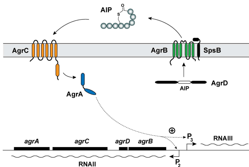
Figure 1. Schematic of the agr system in Staphylococci. The locus is composed of two divergent transcripts called RNAII and RNAIII, driven by the P2 and P3 promoters, respectively. The RNAII transcript is an operon of four genes, agrBDCA , which encodes the core machinery of the system. AgrD is the peptide precursor and is processed and exported through AgrB and SpsB action at the cytoplasmic membrane. SpsB is the house-keeping type I signal peptidase. At the threshold concentration, autoinducing peptide (AIP) binds to the AgrC receptor, a membrane-bound histidine kinase. AIP binding activates the AgrC kinase, resulting in phosphorylation of the AgrA response regulator and activation of the P2 and P3 promoters. AgrA also activates the PSM \alpha and PSM \beta promoters (not shown). This figure is an adaption of the version reported by Thoendel et al. 66 . Reprinted with permission from reference 66 . Copyright 2009 The American Society for Biochemistry and Molecular Biology, Inc.
