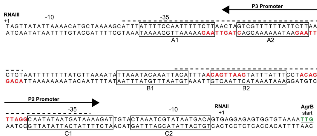
Figure 12. The agr P2-P3 intergenic region. RNAII and RNAIII transcriptional start sites are marked with a +1. Direct repeats recognized by AgrA are colored red while areas protected from DNaseI cleavage by AgrA are indicated with a dashed line above the sequence. Boxes indicate SarA binding sites as reported by Rehtin et al. 143 .
