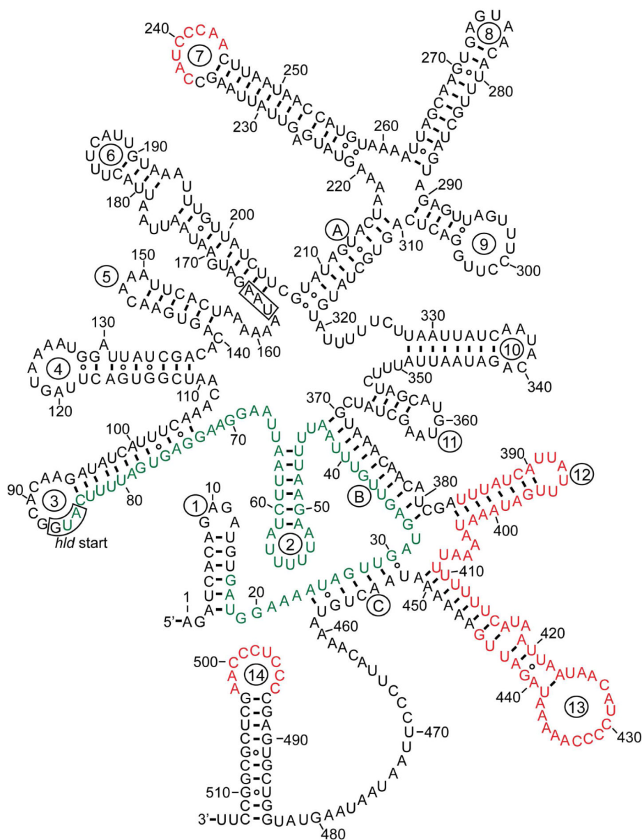
Figure 13. Secondary structure of S. aureus RNAIII. RNAIII hairpins are designated with circled numbers while letters signify long range interactions that establish general domains. hld start and stop codons are boxed. Nucleotides that basepair with and activate hla translation are colored green. Nucleotides demonstrated to inhibit translation of genes are red. This figure is an adaptation from Benito et al. 116 . Reprinted with permission from Reference 116 . Copyright 2000 Cold Spring Harbor Laboratory Press.
