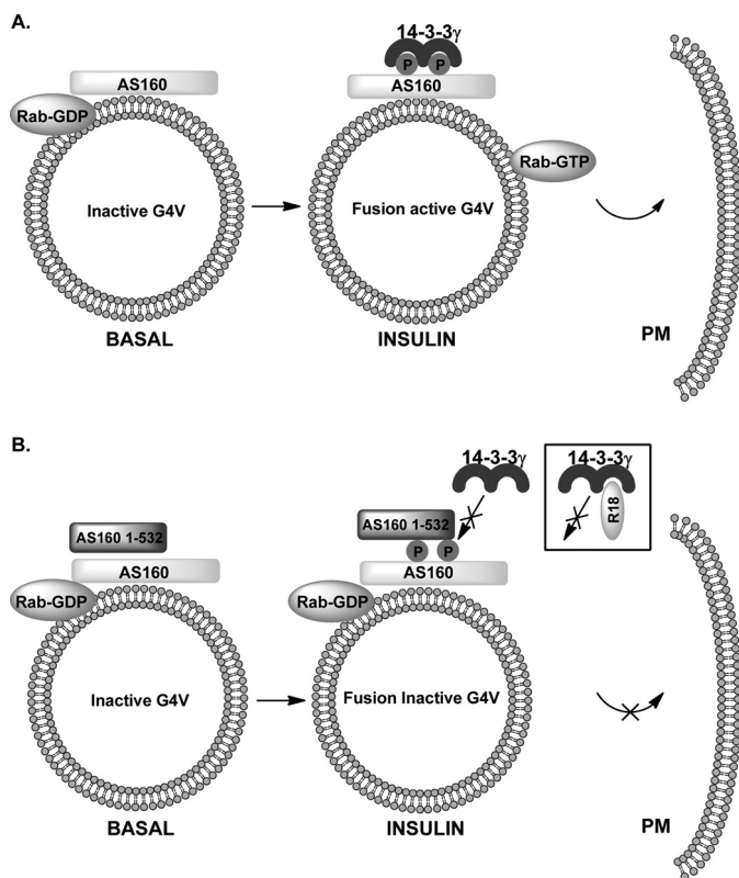
FIGURE 6. Model for inhibitory effects of AS160 N-terminal PTB domain constructs and 14-3-3-quenching reagents on GLUT4 vesicle fusion. A , insulin-stimulated generation of fusion-active GLUT4 vesicles (G4V). Insulin action leads to AS160 phosphorylation and 14-3-3 \gamma binding and consequently generation of a GLUT4 vesicle Rab in an active GTP-loaded form. B , proposed mechanism for fusion inhibition by the N-terminal tandem PTB domain construct AS160(1–532). It is proposed that heterodimer formation with full-length AS160 prevents 14-3-3 \gamma binding. The R18 peptide prevents 14-3-3 \gamma binding through direct quenching reaction. PM , plasma membrane.
