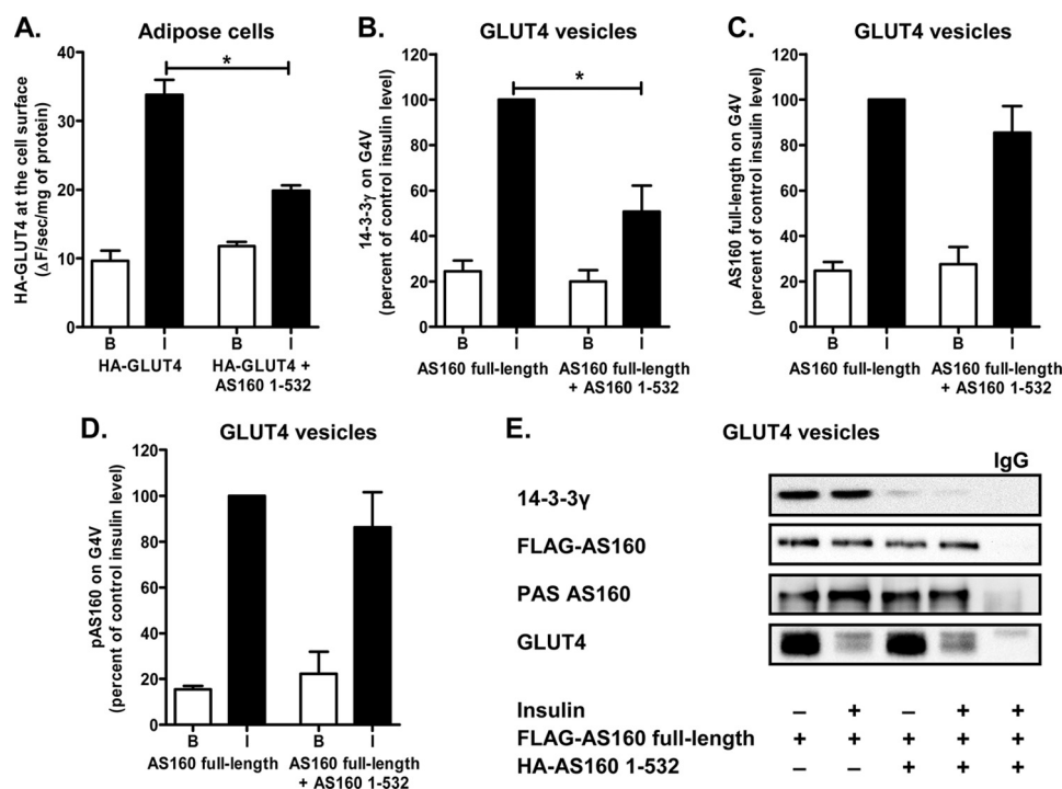
FIGURE 4. AS160(1-532) interacts with full-length AS160 and reduces the relative amount of 14-3-3 \gamma bound to AS160 and associated with GLUT4 vesicles. A , primary rat adipocytes were cotransfected by electroporation with HA-tagged GLUT4 and FLAG-tagged AS160(1-532). After 5 h of expression, cells were maintained in the basal state ( B ) or stimulated with 60 nM insulin ( I ). HA-GLUT4 present at the cell surface was detected after incubating the intact cells with anti-HA antibody for 1 h and detection using a \beta -galactosidase-coupled secondary antibody generating a fluorescent product. Results are means \pm S.E. from four replicates from a single experiment representative of two independent experiments. *, p < 0.05 (comparison of HA-GLUT4 alone versus HA-GLUT4 plus FLAG-AS160(1-532)). B–D , primary rat adipocytes were cotransfected by electroporation with FLAG-tagged full-length AS160 and HA-tagged AS160(1-532). After 12 h of expression, cells were left unstimulated or stimulated with 60 nM insulin and then homogenized. GLUT4 vesicles (G4V) were immunisolated, and the relative amounts of 14-3-3 \gamma ( B ), AS160 ( C ), and phosphorylated AS160 (pAS160; D ) were detected by immunoblotting with anti-14-3-3 \gamma , anti-AS160, and anti-PAS antibodies, respectively. Results are means \pm S.E. from three independent experiments. E , representative immunoblots for data quantified in B–D . *, p < 0.05 (comparison of FLAG-AS160 alone versus FLAG-AS160 plus HA-AS160(1-532)).
