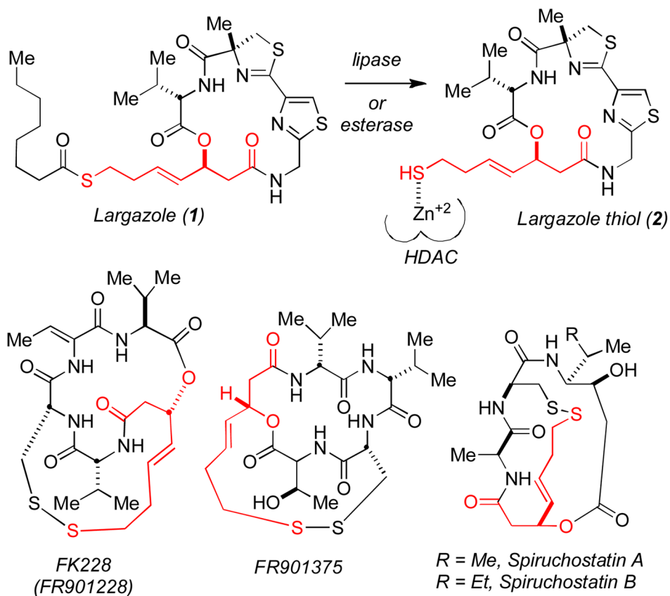
Figure 1. Structure of largazole (1), largazole thiol (2) and several known macrocyclic HDACi natural products containing the ( S )-3-hydroxy-7-mercaptohept-4-enoic acid moiety.
