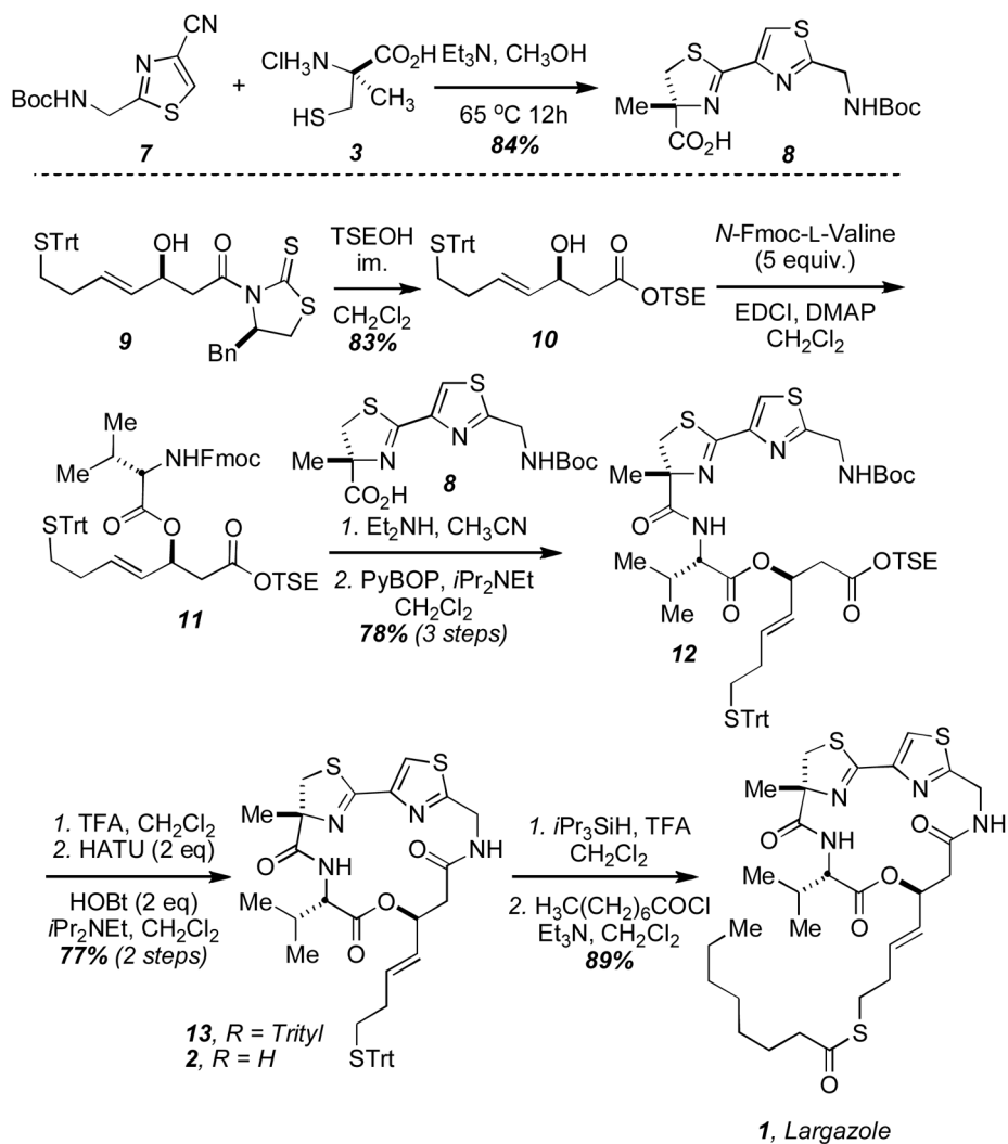
Scheme 1. The total synthesis of largazole ( 1 ) and largazole thiol ( 2 ).
