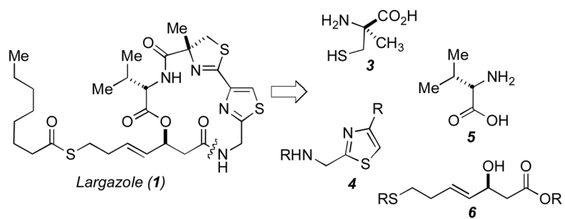
Figure 2. Synthetic strategy to assemble largazole.
