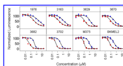
Figure 5. Antiproliferative effects of largazole (red) and largazole thiol (blue). Effects on cell viability were evaluated using a panel of human malignant melanoma cell lines, using the standard, surrogate measurement of ATP content (Cell TiterGlo; Promega) in 384-well plate format. Replicate measurements were normalized to vehicle-only controls and IC_{50} calculations were performed by logistic regression (Spotfire DecisionSite). Largazole demonstrates a potent antiproliferative effect ( IC_{50} 45 nM – 315 nM) compared to largazole Thiol ( IC_{50} 360 nM – 2600 nM).
