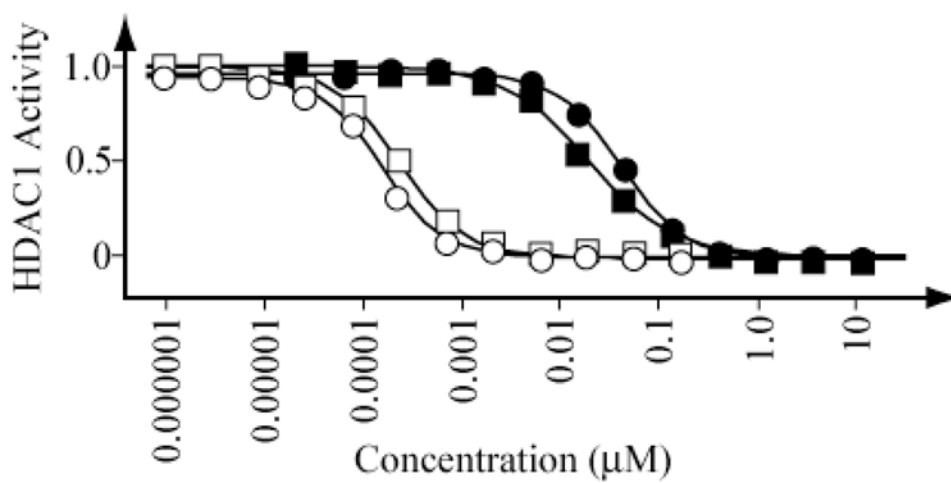
Figure 3. Inhibition of HDAC1 by largetazole (filled circles), largetazole thiol (open circles), SAHA (filled squares) and FK228 (open squares).
