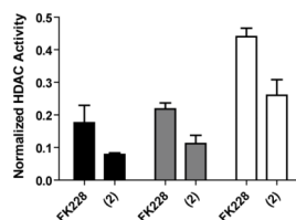
Figure 4. Comparative profiling of FK228 and the largazole thiol ( 2 ). Dose-ranging studies of FK228, largazole and the largazole thiol were performed against Class I HDAC proteins using the described kinetic, homogeneous assay (see Supporting Information). As a comparative measure of potency, compounds were studied in triplicate at a standard concentration (0.6 nM). Averaged data are presented for inhibition of HDAC1 (black), HDAC2 (gray) and HDAC3/NCoR2 (white). Error bars reflect one standard deviation from the mean.
