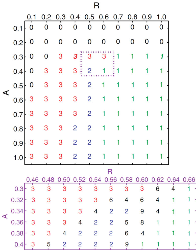
Figure 4. Top panel: finite fast pulse trains computed from the initial perturbation (3) with \Delta = 0.1 for different values of A and R when a_v = 0.5 . The integers correspond to the number N of pulses in the wave train, the bold italic fonts corresponding to the solutions described in fig. 3. Bottom panel: variation in N in the vicinity of the extinction boundary, in the region indicated by the small rectangle in the top panel. The numerical integration of eqs. (1) was performed with \Delta x = 0.005 and Neumann boundary conditions on an L = 50 domain.
