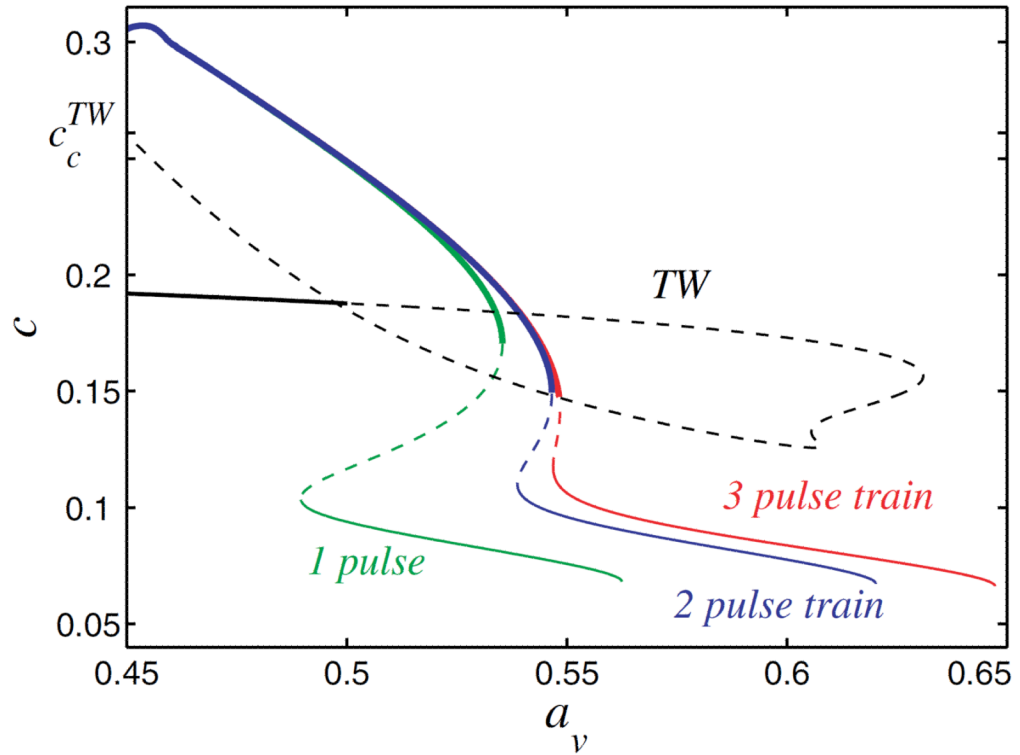
Figure 5. (Color online) The speed c of the fast (heavy colour lines) and slow (thin colour lines) pulse trains as a function of a_v , together with the phase speed of traveling wave (TW) states. Only three branches of traveling pulse trains are shown. The phase speed of the TW lies between the speeds of the fast and slow pulse trains. Solid (dashed) lines indicate stable (unstable) states. The accumulation of the saddle-nodes of the fast pulse trains ( a_v \approx 0.55 ) defines the upper boundary of the shaded region displayed in fig. 1. The pulse trains were computed in a comoving frame, on a periodic domain with L = 100 .
