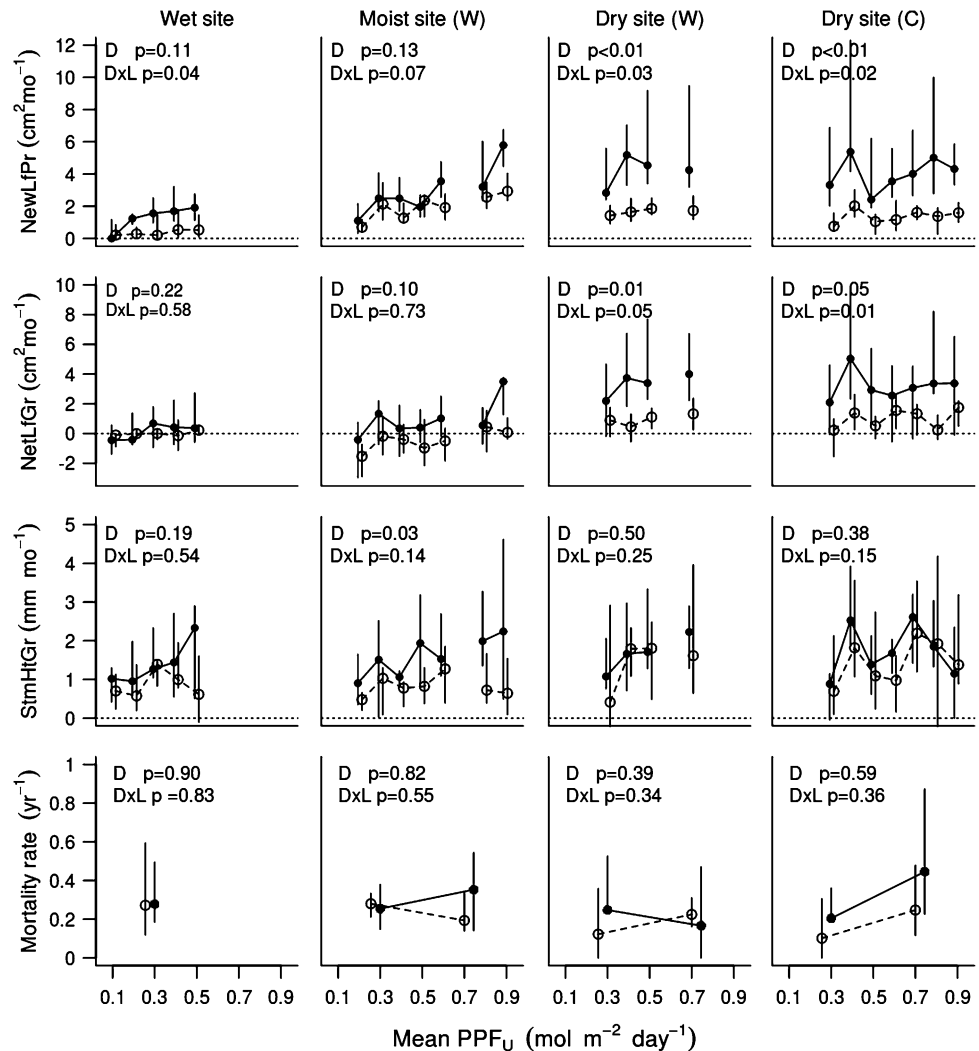
Fig. 4 Comparison of the performance of wet- ( filled circle ) versus dry- ( open circle ) distribution species grown at different understory light levels in wet, moist and dry sites , with ( W ) and without water supplementation ( C ). The symbols represent the medians, and vertical bars represent the inter-quartile range for each group of species at each light category. To improve legibility, plots with similar light levels were combined by averaging seedling performance within species. For mortality rates, we used only two light categories: less than and more than 0.5 \text{ mol m}^{-2} \text{ day}^{-1} . Only data for uncaged seedlings are reported. The P values in the panels represent the significance of the main effect of distribution on seedling performance ( D ) and the distribution \times light interaction ( D \times L ), using linear mixed-effect models for the growth variables and Cox models for mortality
