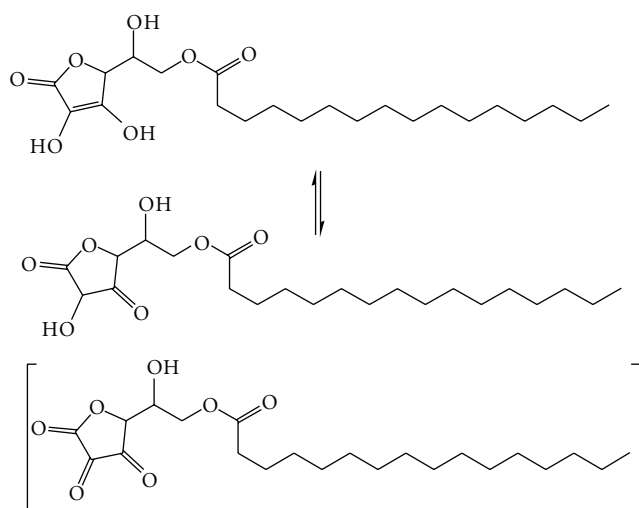
FIGURE 3: Tautomerization of ascorbyl palmitate. Structure of dehydroascorbyl palmitate is shown in parentheses.
