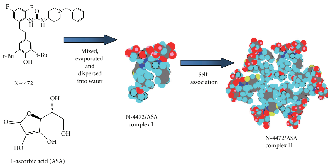
FIGURE 5: Schematic representation for proposed structure of N-4472/ASA surface active complex formation and the subsequent self-association used to form the stable nanosuspension.
