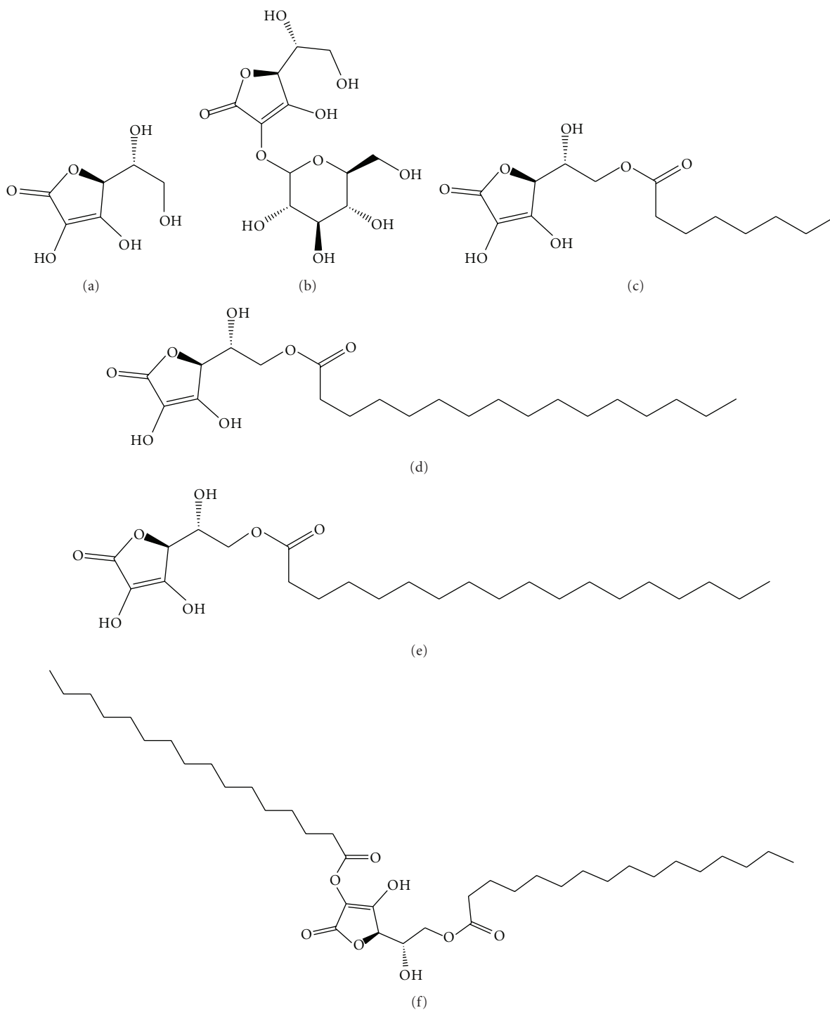
FIGURE 1: Chemical structures of ascorbic acid and its derivatives: (a) ascorbic acid (ASA), (b) ascorbyl-2-glucoside (ASC-G), (c) ascorbyl-6-octanoate (ASC-8), (d) ascorbyl-6-palmitate (ASC-P), (e) ascorbyl-6-stearate (ASC-S), and (f) ascorbyl-2,6-dipalmitate (ASC-DP).
