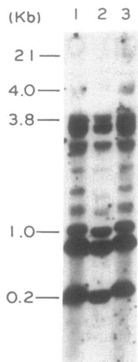
Figure 1. Southern blot hybridization of EcoRI digested genomic DNA (run on 1.0% agarose gel) with ribosomal RNA labelled with [ \gamma^{32} P]ATP using T4 polynucleotide kinase. Lanes 1, 2 and 3 contain different clinical isolates of M.tb.
