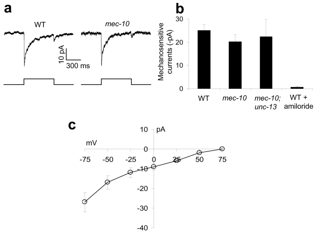
Figure 6. An amiloride-sensitive channel(s) mediates mechanosensitive currents in PVD (a) Mechanical stimulation evokes mechanosensitive currents in PVD. Such currents persisted in mec-10(tm1552) . Clamping voltage: -75 mV. Touch was directed to the primary dendrite of PVD. Displacement: 20 \mu\text{m} . A 10 \mu\text{m} displacement was needed to evoke mechanosensitive currents in PVD, a much higher threshold than that in PDE. PVD in mec-10(tm1552) animals displayed a similar sensitivity (threshold). (b) Bar graphs. Touch-evoked mechanosensitive currents in PVD were sensitive to amiloride ( 200 \mu\text{M} ) but persisted in mec-10(tm1552) , as well as in mec-10(tm1552); unc-13(e51) double mutant animals. n \geq 5 . Error bars: SEM. (c) I-V relations of mechanosensitive currents in PVD. n \geq 5 . Error bars: SEM.
