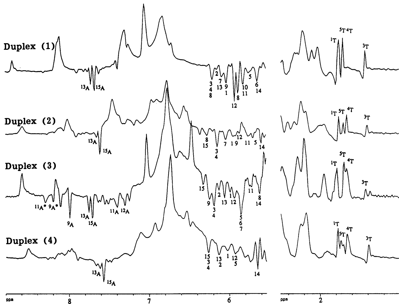
Figure 3. Proton NMR spectra showing NOEs through the cross section of the ROESY 11 spectrum along the f_2 ( \delta 9.0–5.5 ppm and \delta 2.5–1.0 ppm) at the f_1 frequency of the water line with the spinlock duration of 0.06 s for duplexes (1)–(4). The spectra were baseline-corrected in both dimensions using polynomials and also corrected for the excitation profile, \sin^3[2\pi\tau\omega(\delta-\delta_{\text{off}})] 11 , along the \omega_2 frequency axis, where \tau is the delay (187 \mu s), \omega is the frequency of spectrometer (500.13 MHz), \delta is the chemical shift in ppm, \delta_{\text{off}} is the chemical shift of the carrier frequency on water. The upfield region from 2.5–1.0 ppm was inverted for improved readability. Resonance assignments for the H1' protons in \delta 6.5–5.5 ppm region are indicated by the arabic numbers which are identical with the nucleotide number in the DNA sequence (1)–(4). Resonance assignments 5 for the aromatic H2 adenine protons (in \delta 9.0–7.0 ppm region) and methyl thymine protons (in \delta 2.0–1.0 ppm region) are indicated by the nucleotide number and base sequence whereas the aromatic H8 adenine protons are additionally labelled by symbol (*). See ref. 14 for the assignments of the signs of the cross-peaks and ref. 18 for the control experiments supporting the direct magnetization transfer between H2A and bound water.
